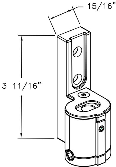
ADJUSTER KNUCKLE
