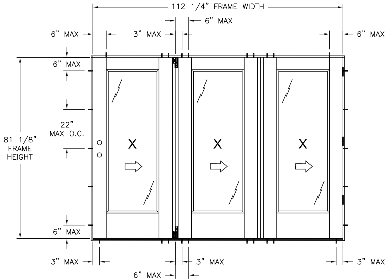
MIRAVISTA FOLDING DOOR SYSTEM W/MASONITE PANELS EXTERIOR VIEW
