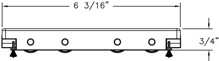
TRUCK ASSEMBLY
