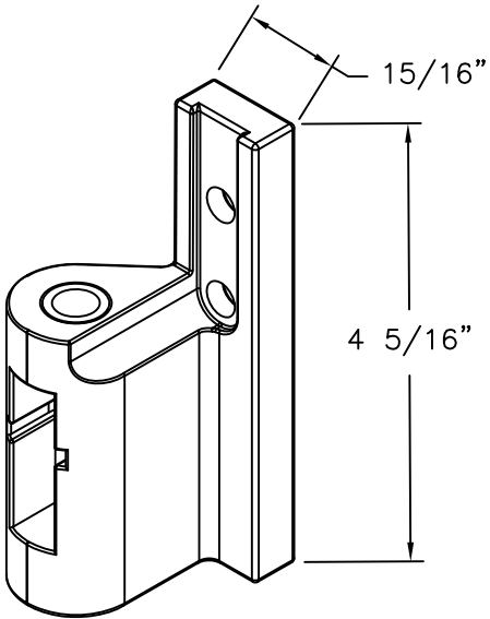
TRUCK KNUCKLE
