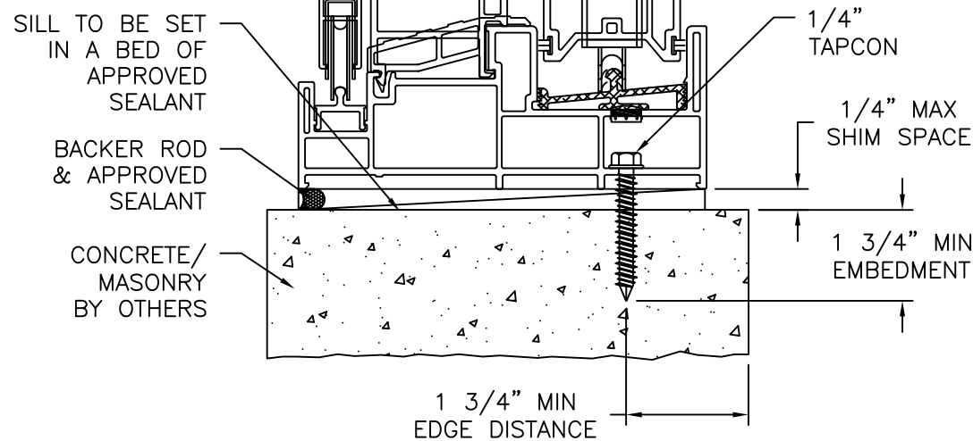
VERTICAL CROSS SECTION CONCRETE/MASONRY INSTALLATION
