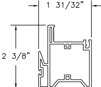
FIXED INTERLOCK RIGID PVC .071" THICK
