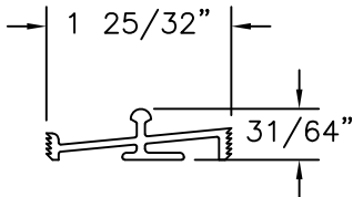
SILL TRACK ALUMINUM 6005-T5, 6105-T5 .069" THICK
