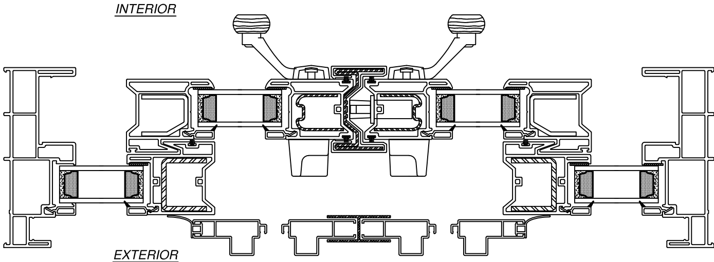
FRAME HORIZONTAL CROSS SECTION
