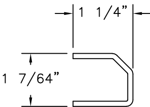
REINFORCEMENT 12GA. G90 GALVANIZED STEEL
