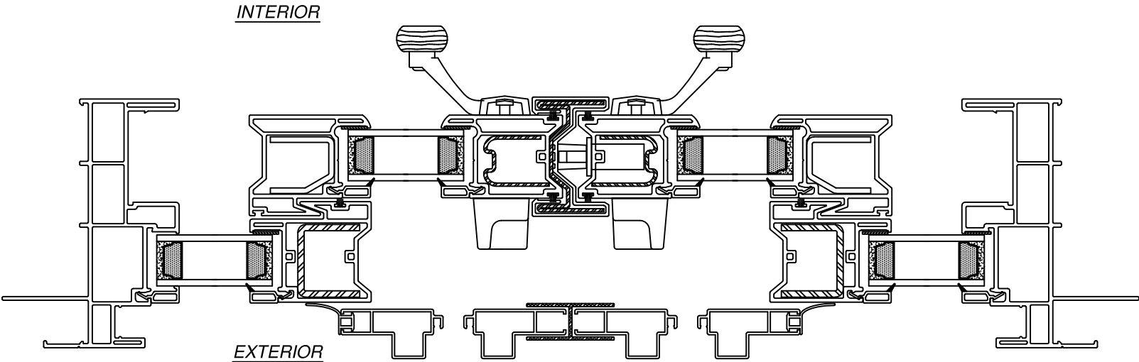
PERIMETER HORIZONTAL CROSS SECTION
