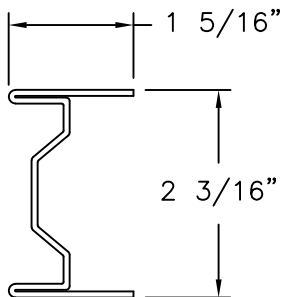
REINFORCEMENT G90 GALVANIZED STEEL .063" THICK
