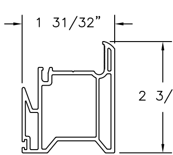
SASH INTERLOCK RIGID PVC .079" THICK
