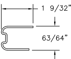
REINFORCEMENT 16GA. G90 GALVANIZED STEEL
