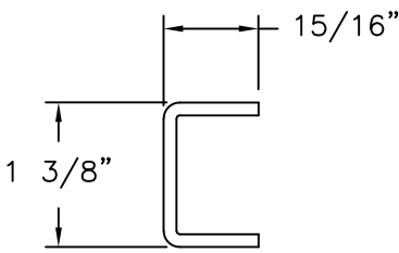
REINFORCEMENT G90 GALVANIZED STEEL .0925" THICK
