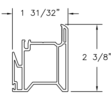
SASH INTERLOCK RIGID PVC .079" THICK
