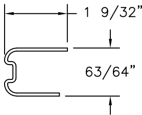
REINFORCEMENT 16GA. G90 GALVANIZED STEEL
