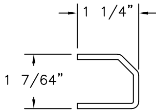
SASH INTERLOCK RIGID PVC .079" THICK
