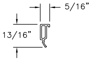
1" GLAZING BEAD RIGID PVC .049" THICK
