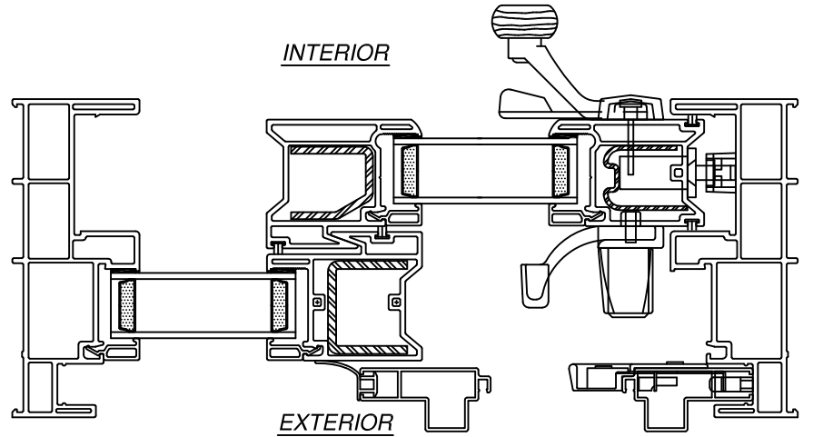
FRAME HORIZONTAL CROSS SECTION
