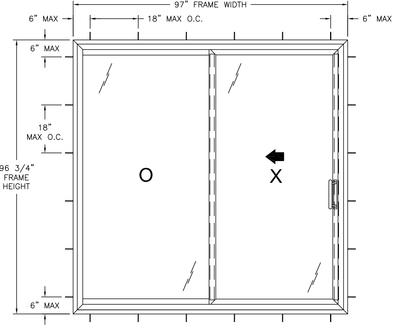
800 SGD EXTERIOR VIEW REINFORCED
