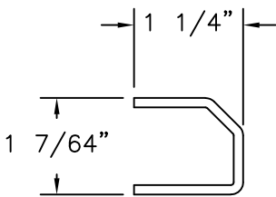
SASH INTERLOCK RIGID PVC .079" THICK
