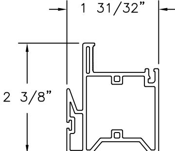
FIXED INTERLOCK RIGID PVC .071" THICK
