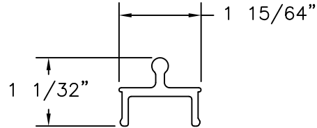
SCREEN TRACK RIGID PVC .130" THICK
