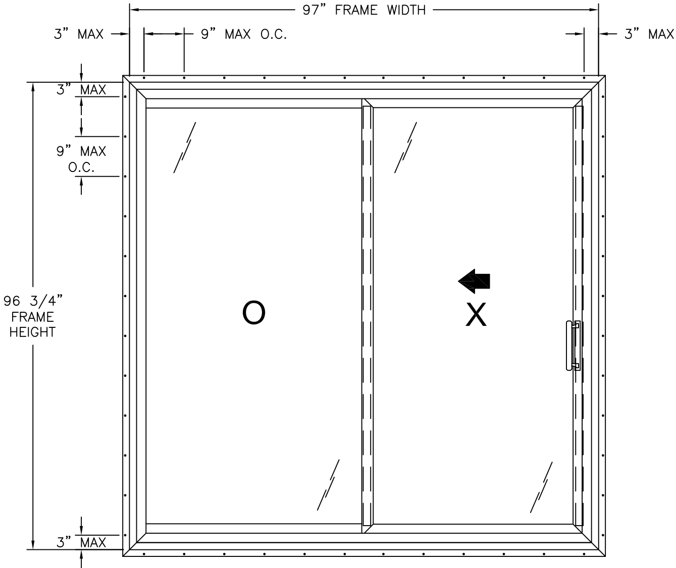
800 SGD EXTERIOR VIEW REINFORCED
