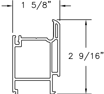
EQUAL GLASS ADAPTER RIGID PVC .079" THICK
