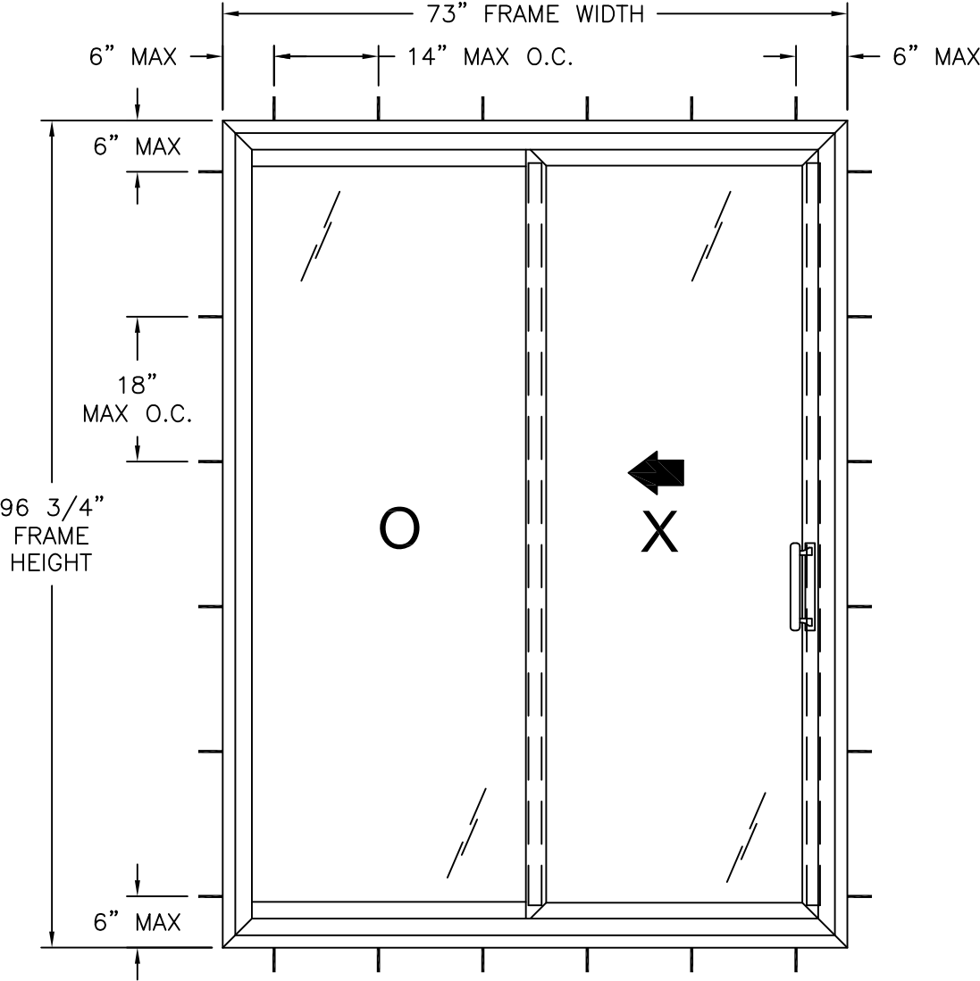
800 SGD EXTERIOR VIEW REINFORCED
