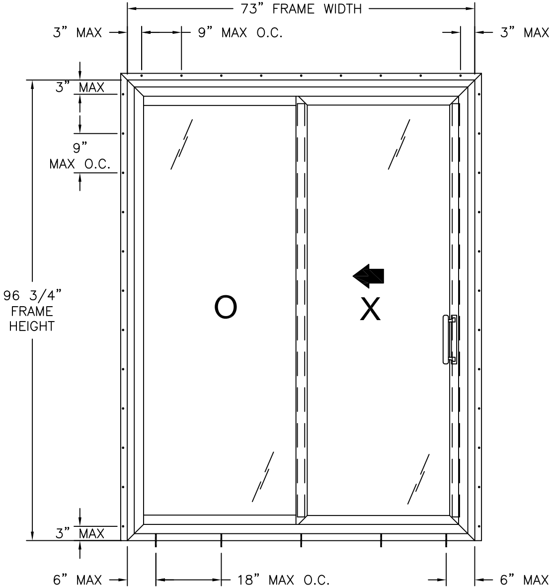
800 SGD EXTERIOR VIEW REINFORCED
