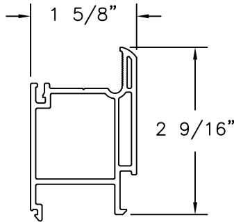
EQUAL GLASS ADAPTER RIGID PVC .079" THICK
