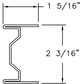
REINFORCEMENT G90 GALVANIZED STEEL .063" THICK
