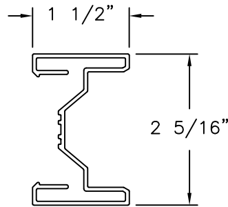
ASTRAGAL RIGID PVC .06" THICK
