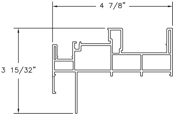
FRAME RIGID PVC .079" THICK
