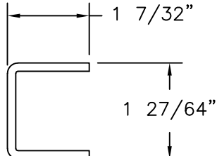
REINFORCEMENT 11GA. G90 GALVANIZED STEEL
