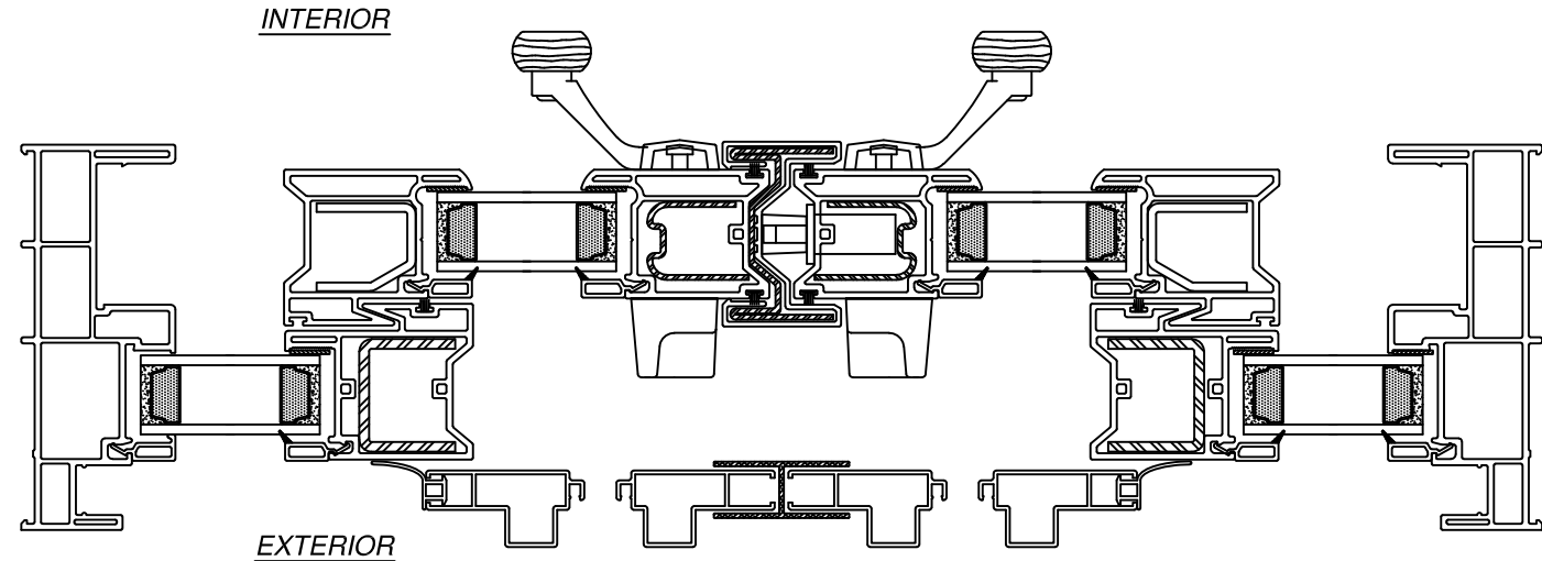
FRAME HORIZONTAL CROSS SECTION
