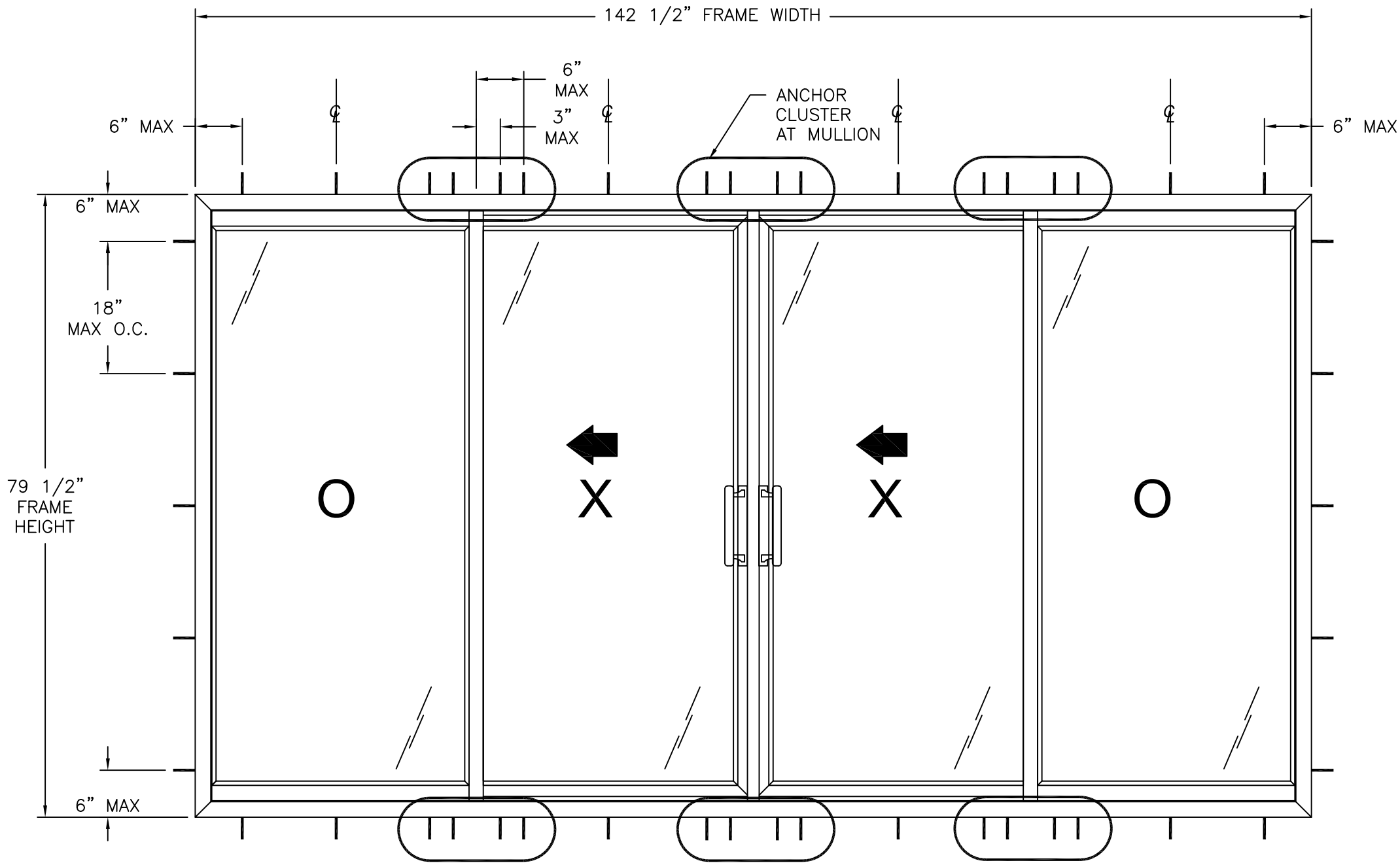
800 SGD EXTERIOR VIEW REINFORCED
