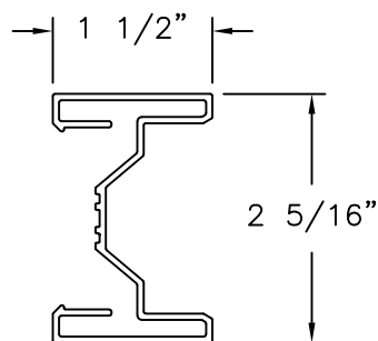
ASTRAGAL RIGID PVC .06" THICK
