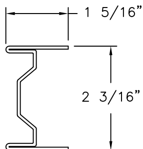
FIXED INTERLOCK RIGID PVC .071" THICK
