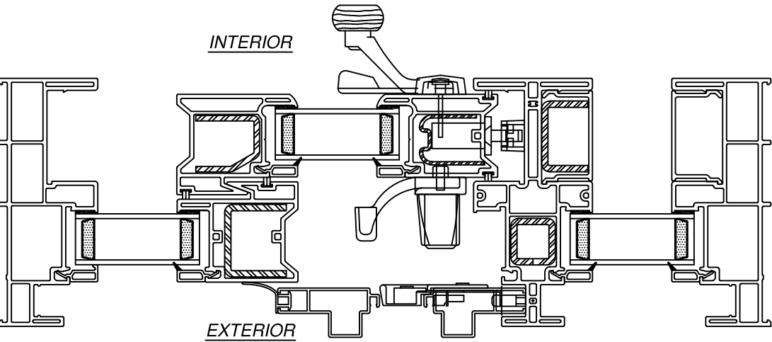
FRAME HORIZONTAL CROSS SECTION
