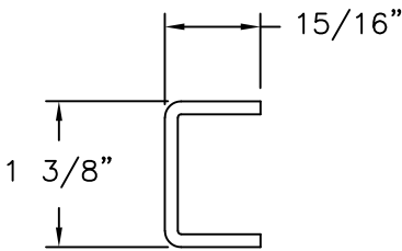
REINFORCEMENT G90 GALVANIZED STEEL .0925" THICK
