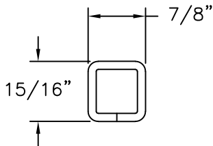
REINFORCEMENT G90 GALVANIZED STEEL .0925" THICK
