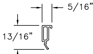
1" GLAZING BEAD RIGID PVC .049" THICK
