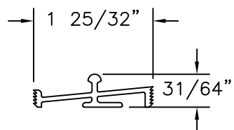
SILL TRACK ALUMINUM 6005-T5, 6105-T5 .069" THICK
