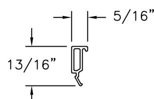
1" GLAZING BEAD RIGID PVC .049" THICK
