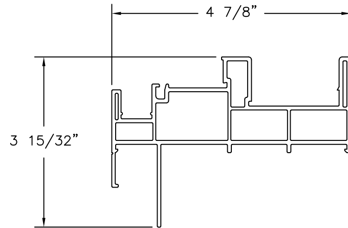
FRAME RIGID PVC .079" THICK
