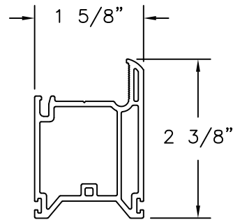
SASH STILE AND RAIL RIGID PVC .079" THICK
