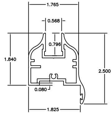
③ CONTINENTAL SASH PERIMETER \frac{7}{16} " GLASS
