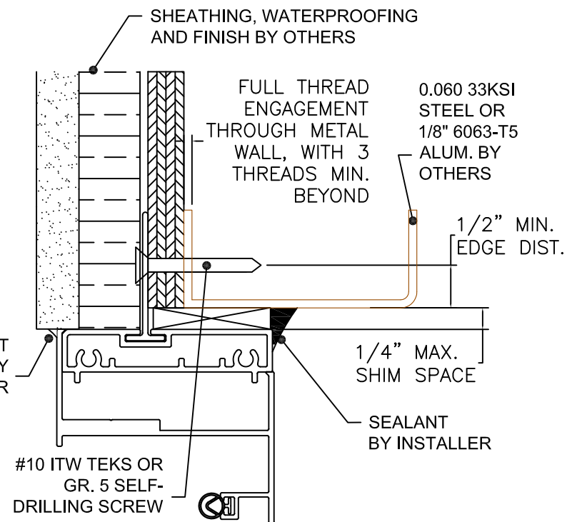
TYPICAL HEAD/SILL INSTALLATION METAL STRUCTURE INSTALLATION
