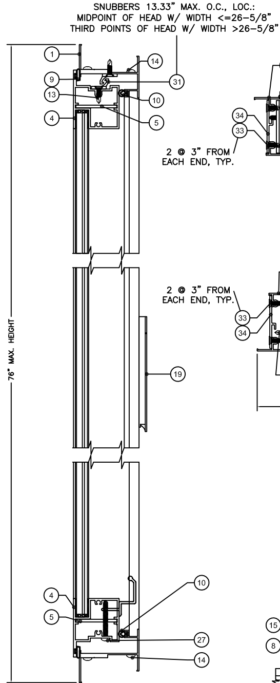
SECTION A
