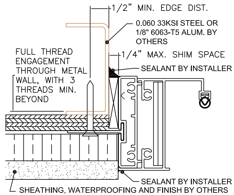
TYPICAL JAMB INSTALLATION METAL STRUCTURE INSTALLATION
