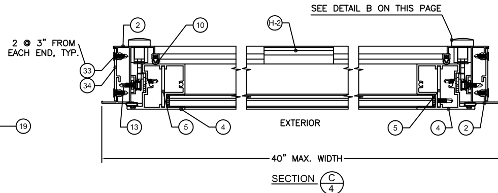
NON-OPERATOR PROJECT OUT CONTINENTAL WINDOW - LINEAL SASH
