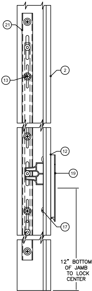
DETAIL A
