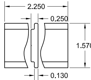
* REINFORCEMENT PLATE DETAIL
