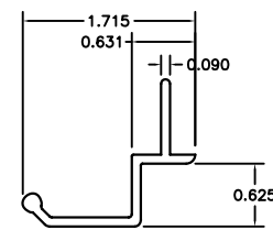
⑥ (H-2) HANDLE LINEAL *
