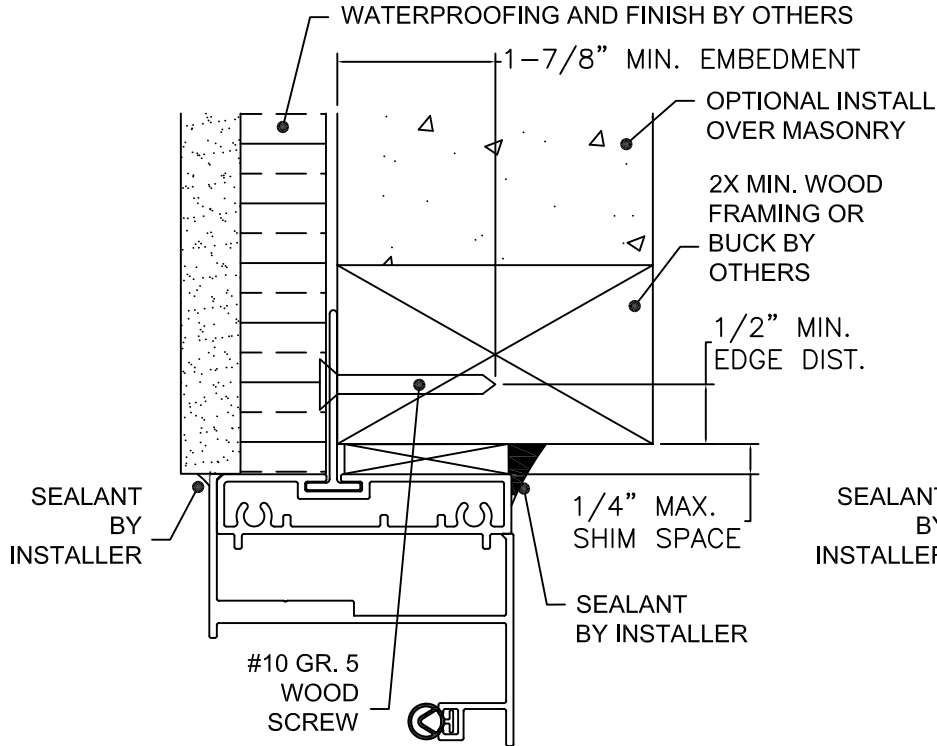
TYPICAL HEAD/SILL INSTALLATION WOOD FRAMING OR 2X BUCK INSTALLATION
