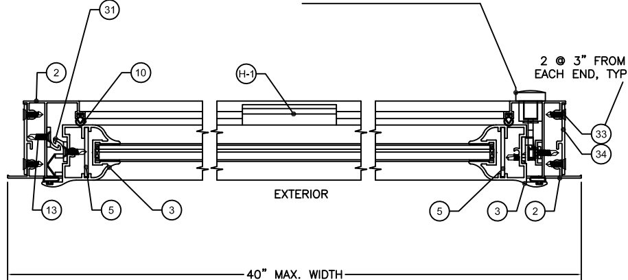
SECTION B 4
