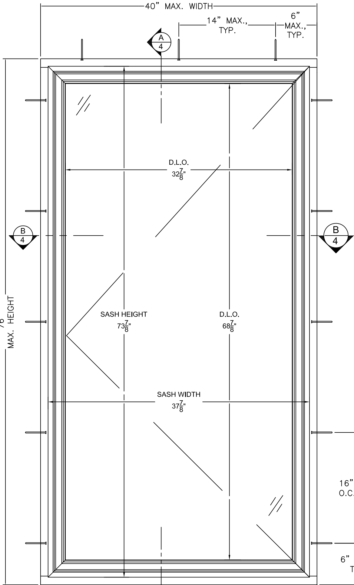
CONTINENTAL EXTERIOR ELEVATION NON-OPERATOR CASEMENT WINDOW
