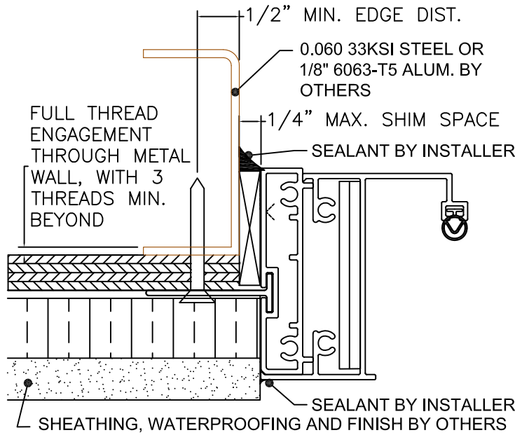
TYPICAL JAMB INSTALLATION METAL STRUCTURE INSTALLATION
