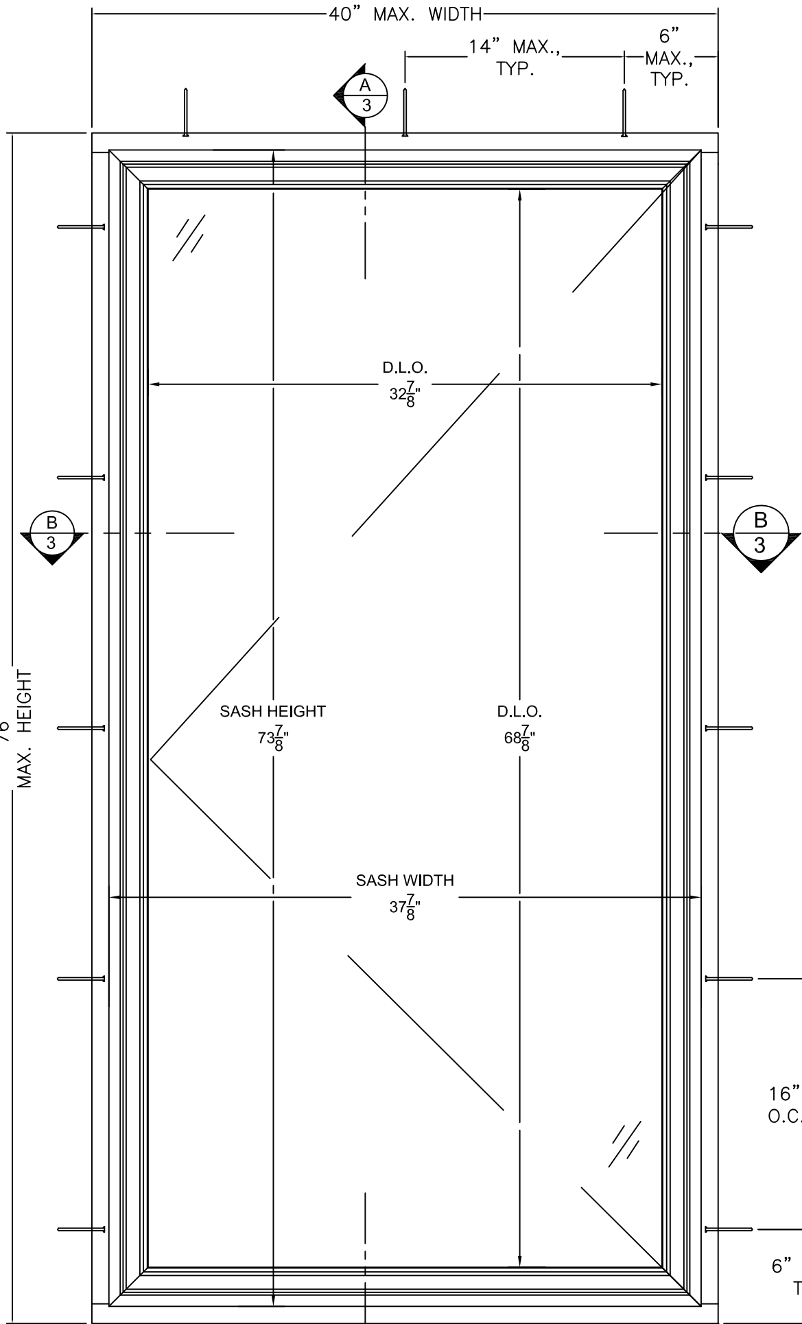
CONTINENTAL EXTERIOR ELEVATION OPERATOR CASEMENT WINDOW
