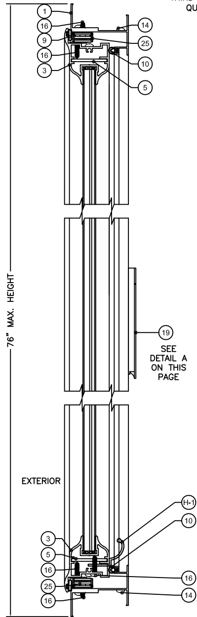
SECTION A 4
