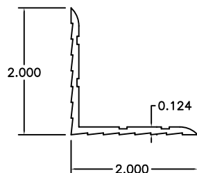
⑤ CORNER LOCK
