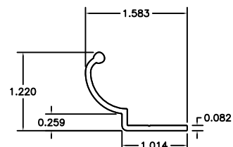
⑥ (H-1) HANDLE CONTINENTAL *
