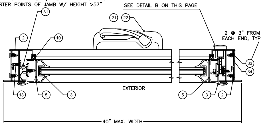
SECTION \frac{B}{3}
