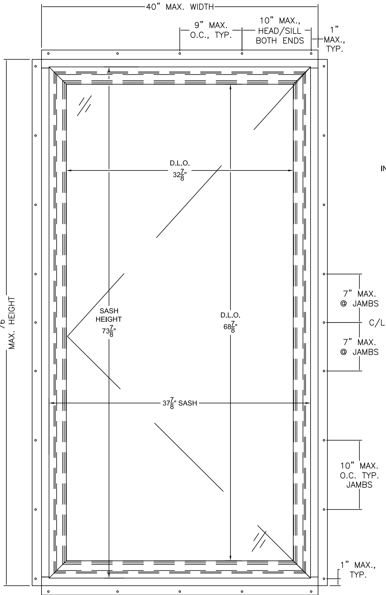
FIN EXTERIOR ELEVATION (APPLICABLE TO ANY SASH / OPERATOR TYPE FOR THIS PRODUCT)
