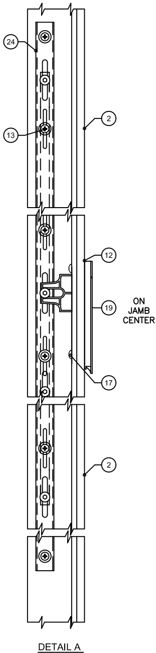
DETAIL A
