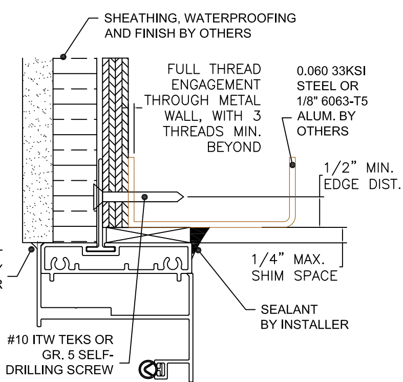
TYPICAL HEAD/SILL INSTALLATION METAL STRUCTURE INSTALLATION
