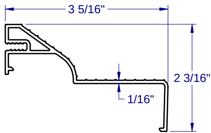
INTERIOR THRESHOLD - 1010
