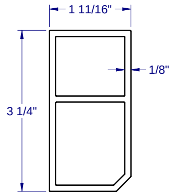
ASTRAGAL REINFORCEMENT - 1014
