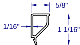
GLAZING BEAD - 6271
