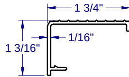
EXTERIOR THRESHOLD - 1011
