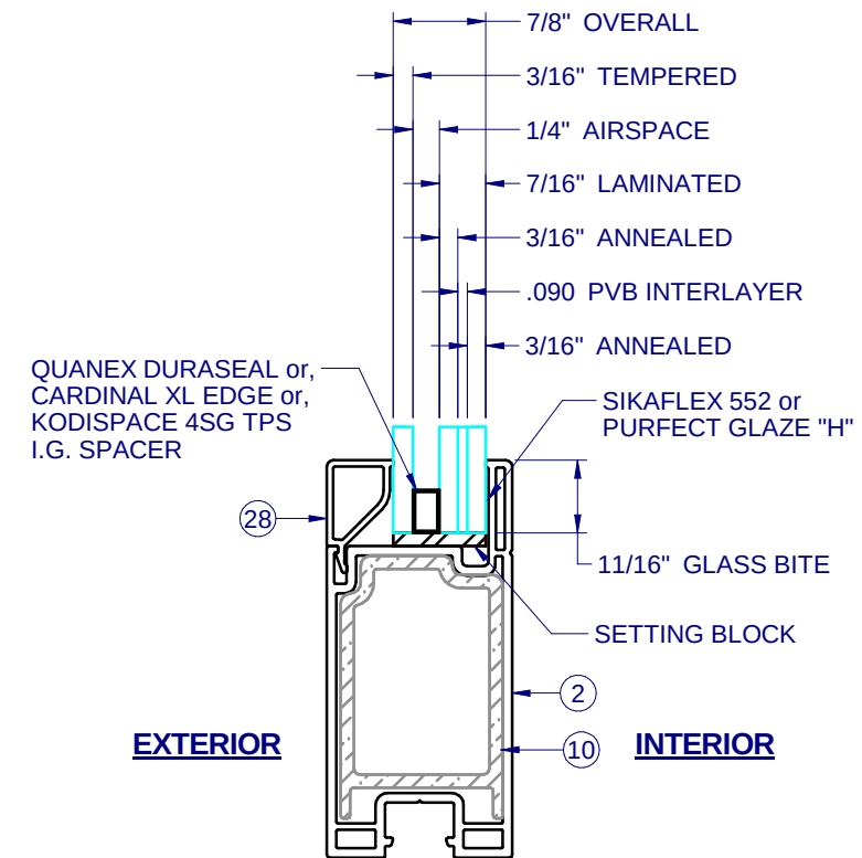
GLAZING DETAIL
