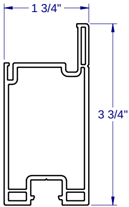
PANEL - 6269
