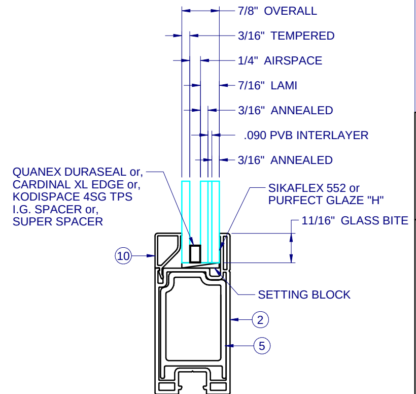
7/8" GLAZING DETAIL
