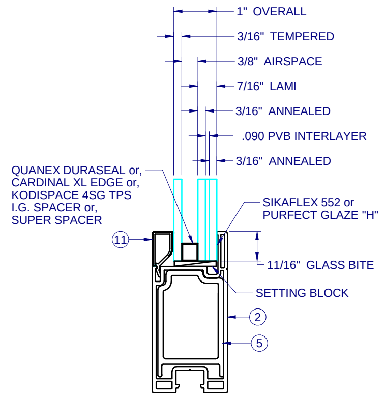
1" ALT GLAZING DETAIL
