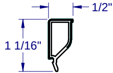
1" GLAZING BEAD - 6276
