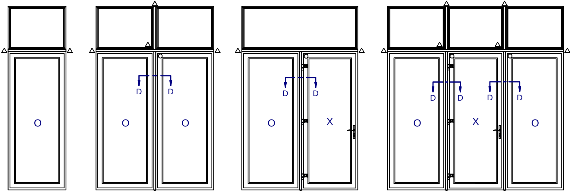
SIDELITE w/ TRANSOM SIDELITE - SIDELITE w/ TRANSOMS SIDELITE - SINGLE SWING DOOR w/ TRANSOM SIDELITE - SINGLE SWING DOOR - SIDELITE w/ TRANSOMS
