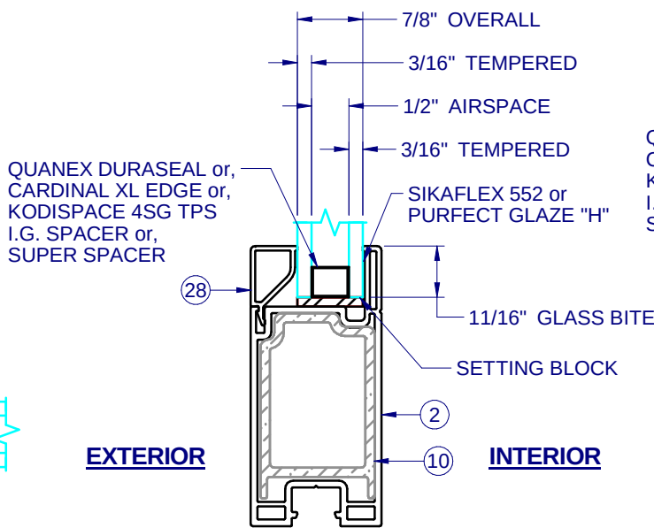
7/8" GLAZING DETAIL
