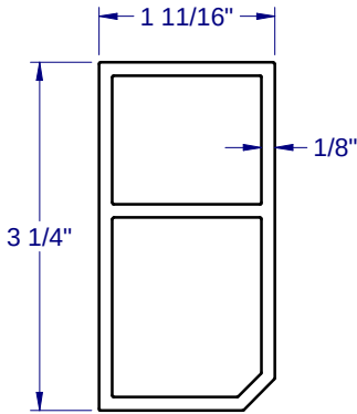
ASTRAGAL REINFORCEMENT - 1014
