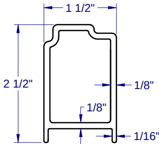
PANEL REINFORCEMENT - 1013
