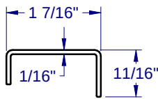
FRAME REINFORCEMENT - 1012
