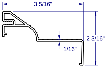
INTERIOR THRESHOLD - 1010
