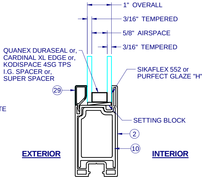
1" ALT GLAZING DETAIL
