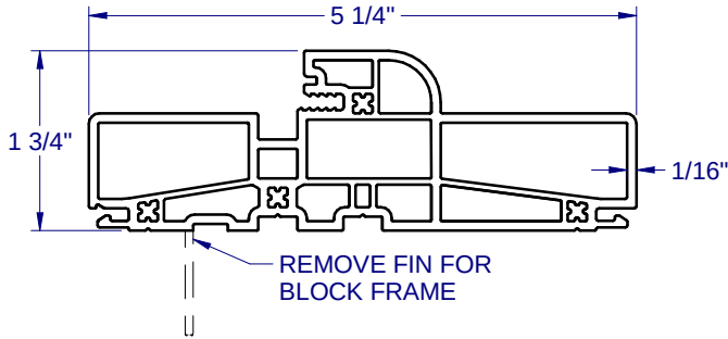
MAIN FRAME - 6268
