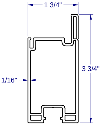
PANEL - 6269
