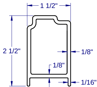
PANEL REINFORCEMENT - 1013
