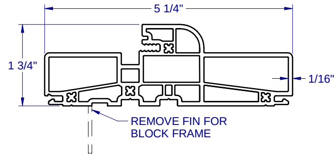
MAIN FRAME - 6268
