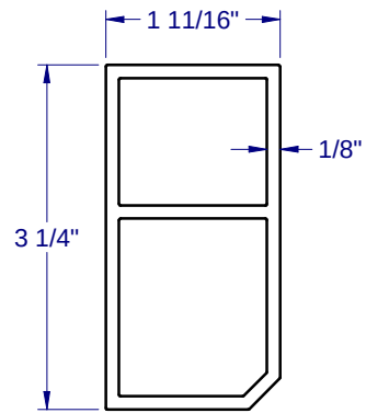
ASTRAGAL REINFORCEMENT - 1014
