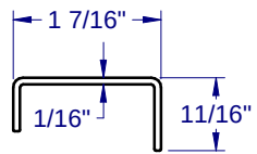
FRAME REINFORCEMENT - 1012
