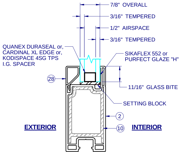
GLAZING DETAIL
