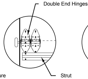
Strut on bottom half of hinge
