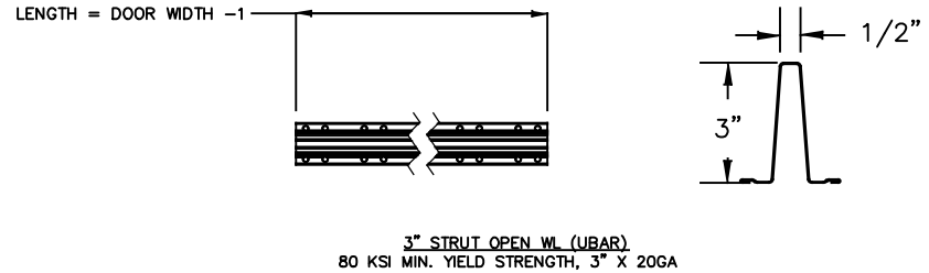
STRUT DETAILS
