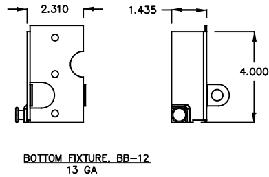
BOTTOM FIXTURE DETAILS
