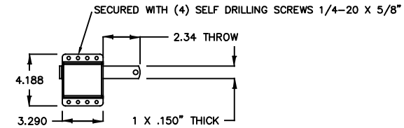
SIDE LOCK ASSY
