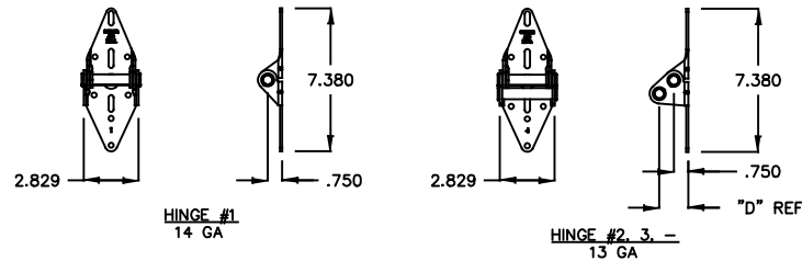
HINGE DETAILS
