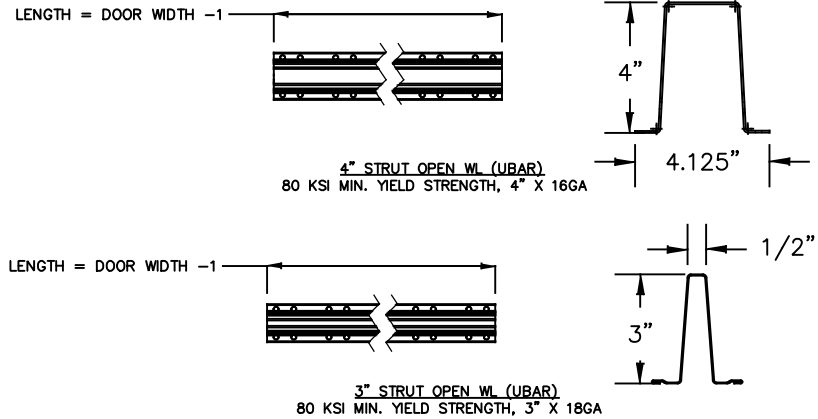
STRUT DETAILS
