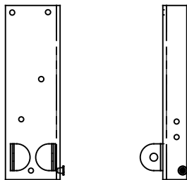
BOTTOM FIXTURE, BB-12 12 GA
