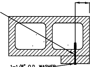
WOOD MOUNTED TO GROUT FILLED MASONRY BLOCK DETAIL
