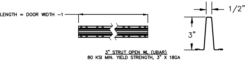
STRUT DETAILS
