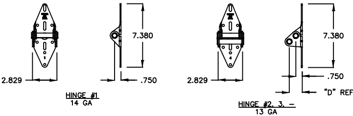
HINGE DETAILS
