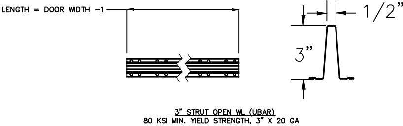
STRUT DETAILS
