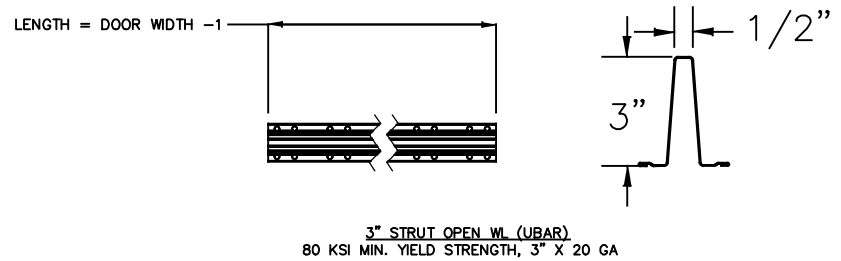
STRUT DETAILS
