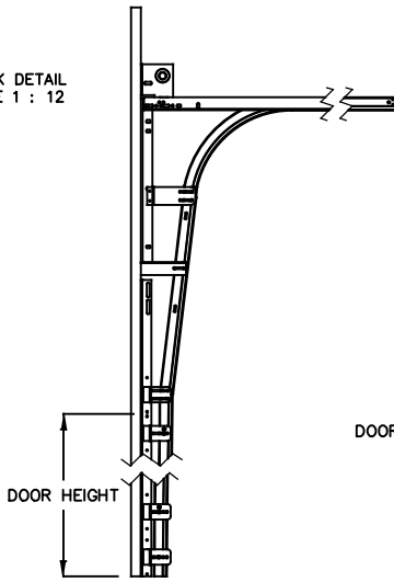
HIGH LIFT TRACK DETAIL
