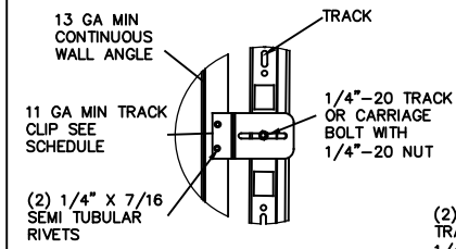
TYPICAL TRACK CLIP RIVETING DETAIL
