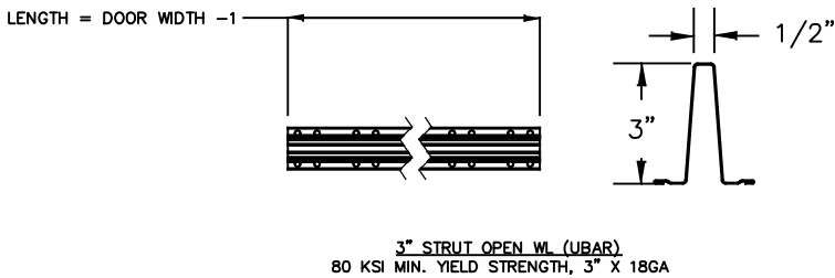
STRUT DETAILS
