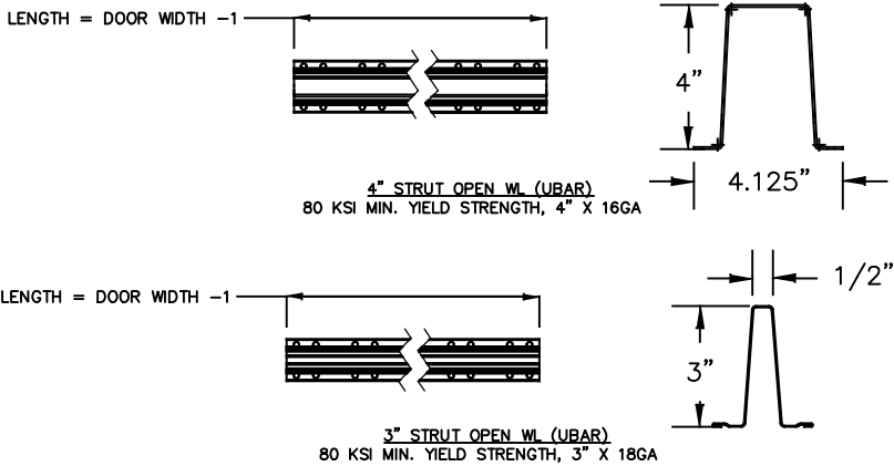
STRUT DETAILS
