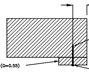
WOOD MOUNTED TO 2500 PSI CONCRETE DETAIL
