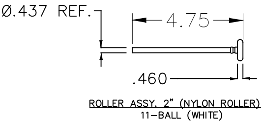
ROLLER STEM ASSY DETAILS
