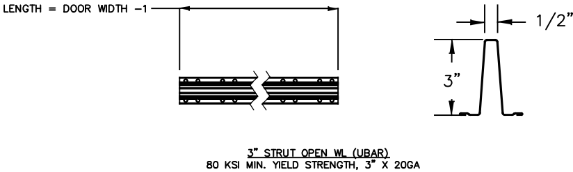
STRUT DETAILS
