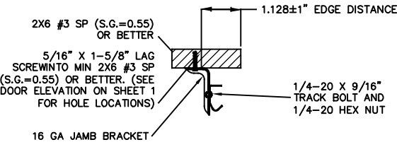
MOUNTING TO WOOD JAMB DETAIL
