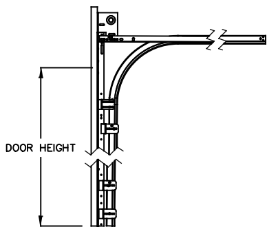
STANDARD LIFT TRACK DETAIL
