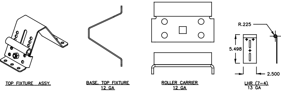
TOP FIXTURE DETAILS
