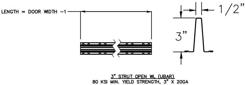
STRUT DETAILS
