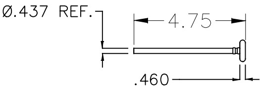
HINGE DETAILS
