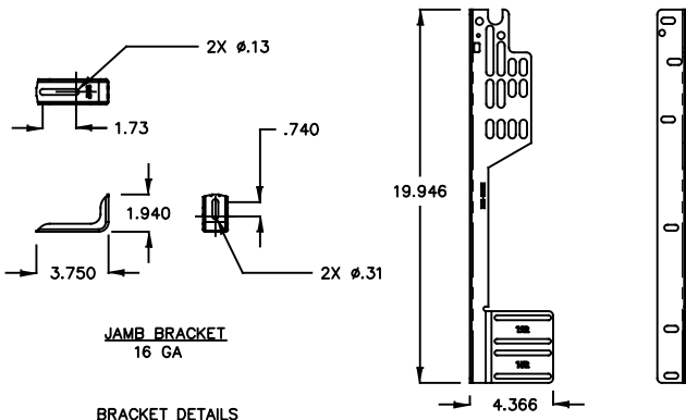
BRACKET DETAILS
