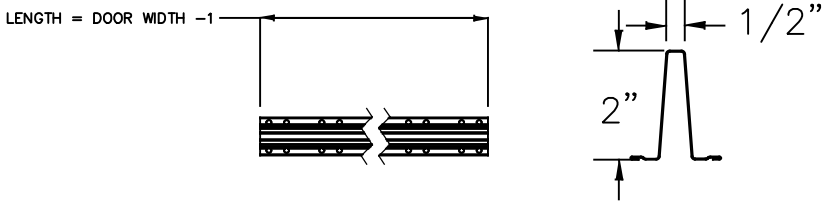
STRUT DETAILS
