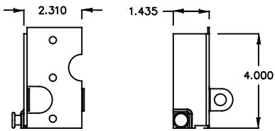
BOTTOM FIXTURE DETAILS
