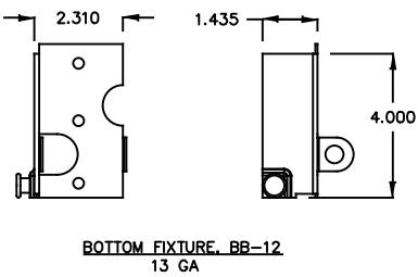
BOTTOM FIXTURE DETAILS
