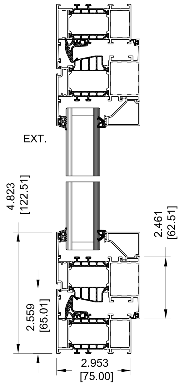
VERTICAL SECTION CASEMENT AND TILT&TURN
