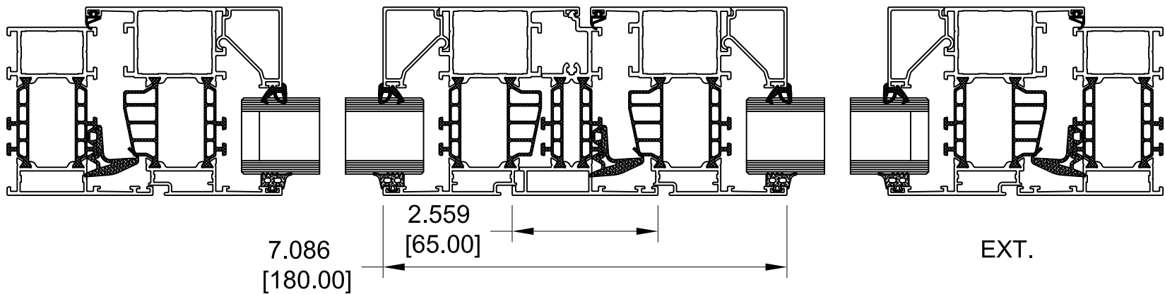
HORIZONTAL SECTION
