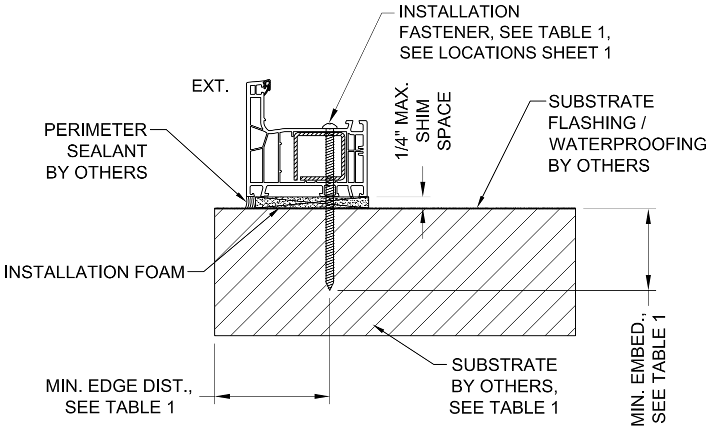
TYPICAL INSTALLATION, HEAD/SILL/JAMB
