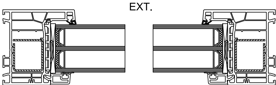
HORIZONTAL SECTION
