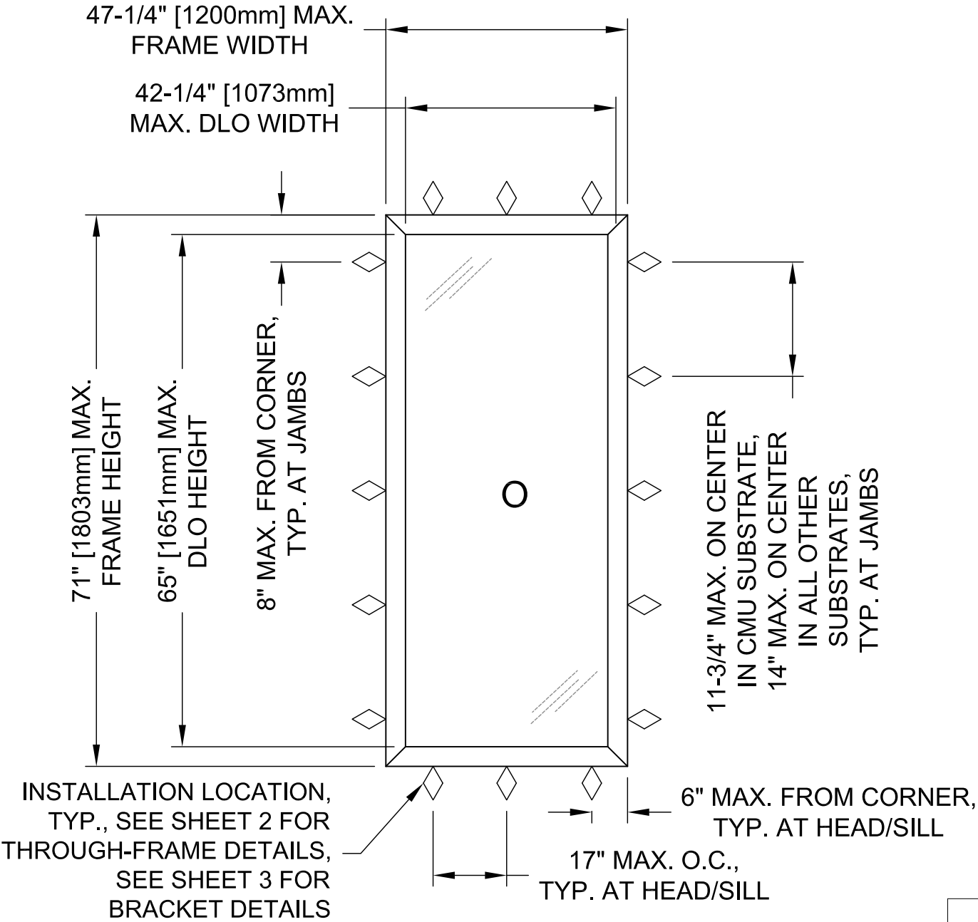
TYPICAL ELEVATION
