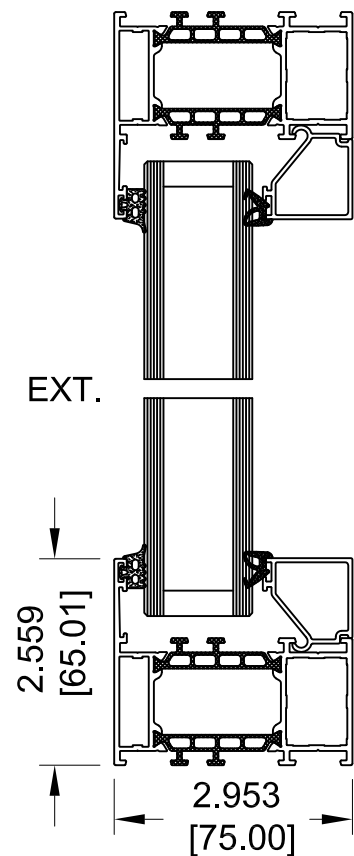
VERTICAL SECTION
