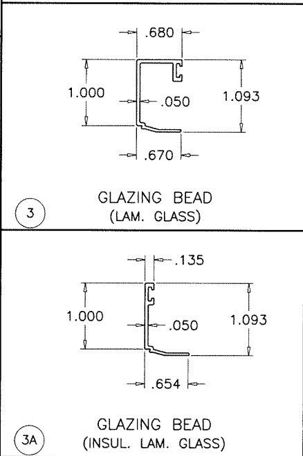
3 GLAZING BEAD (LAM. GLASS)
