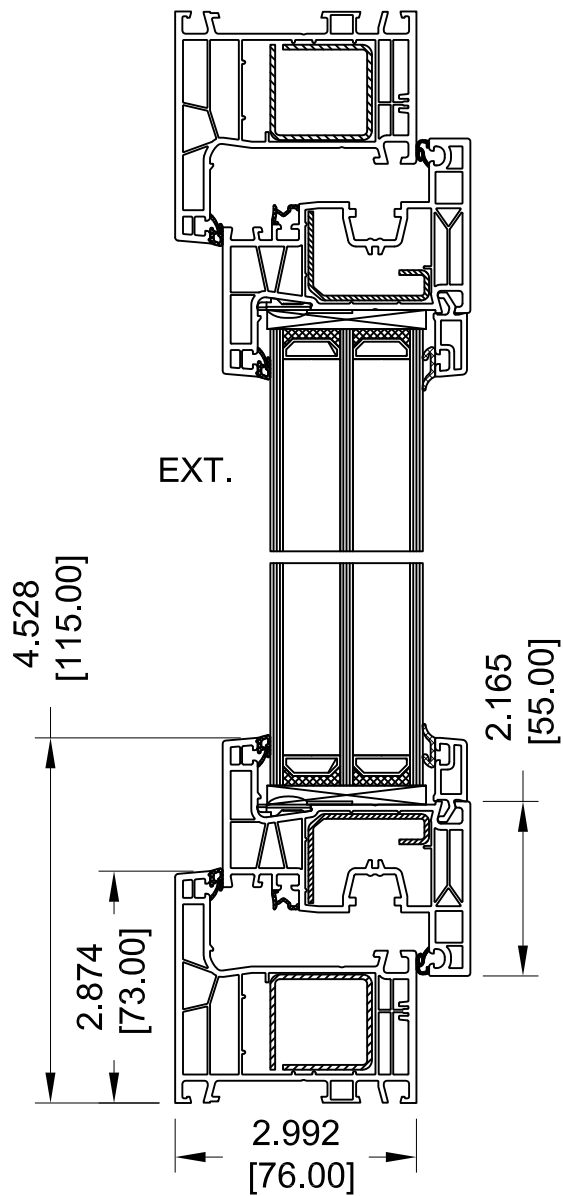
VERTICAL SECTION
