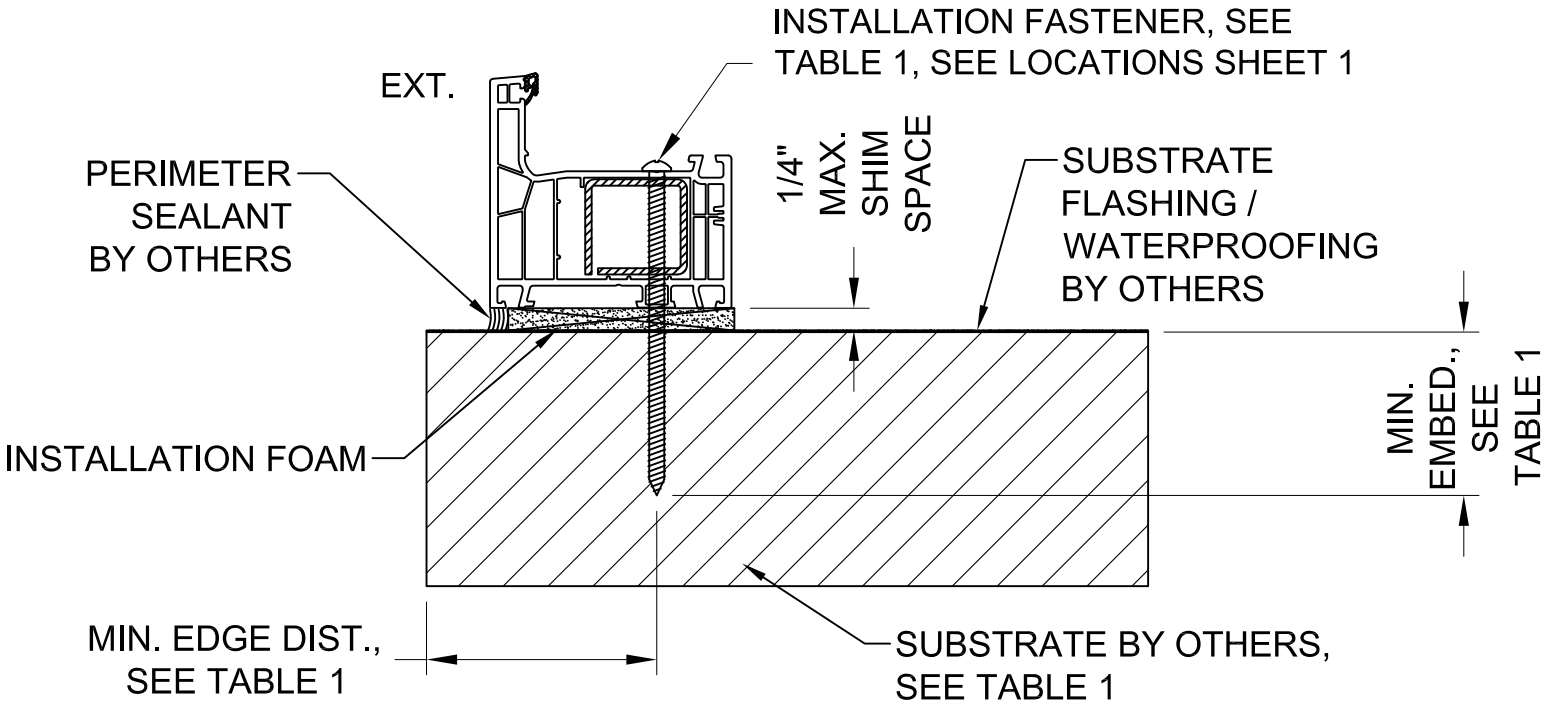
TYPICAL INSTALLATION, HEAD/SILL/JAMB
