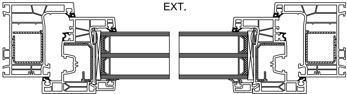
HORIZONTAL SECTION
