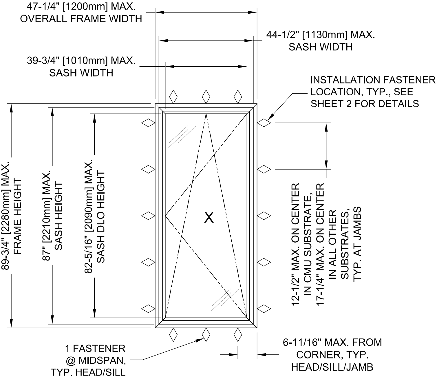
TYPICAL ELEVATION
