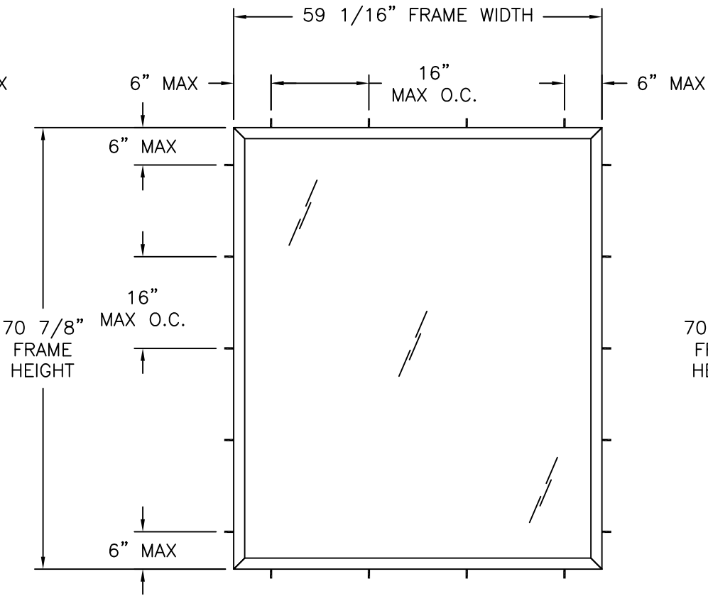
THROUGH FRAME ANCHORING FOR DP RATINGS LOWER THAN 30.0PSF
