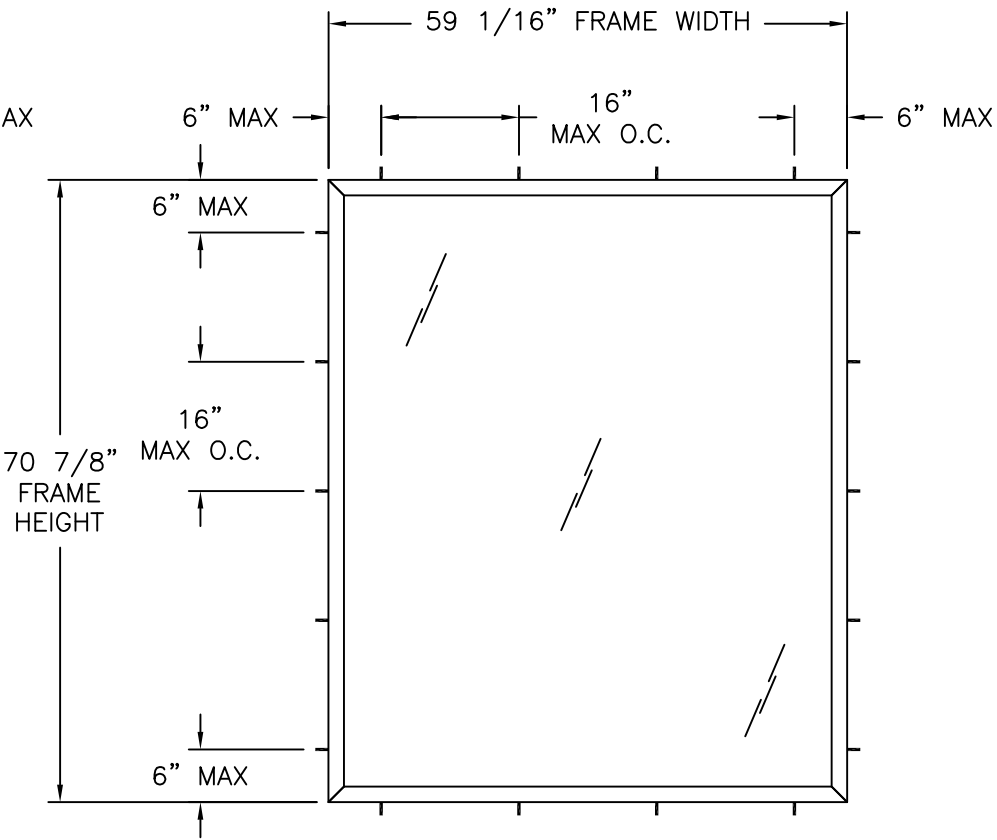
FLAT CLIP OR ANGLE ANCHORING FOR ALL RATINGS
