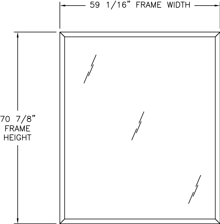
NW FIXED 510 WOOD WINDOW EXTERIOR VIEW
