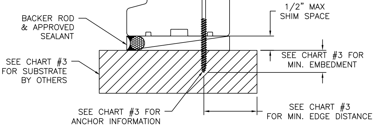
VERTICAL CROSS SECTION
