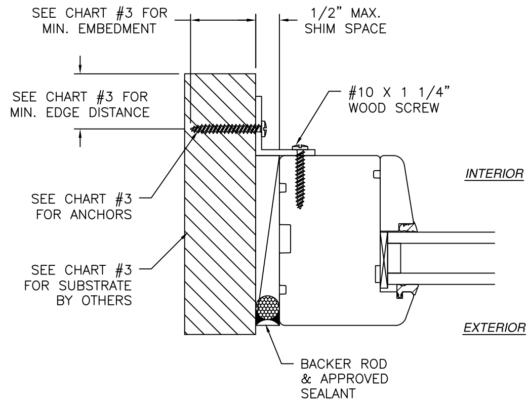
JAMB INSTALLATION DETAIL
