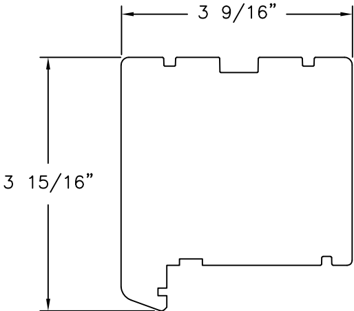
ALTERNATE HEAD AND JAMB 3-4 LAYER OF CROSS GRAINED SOLID WOOD
