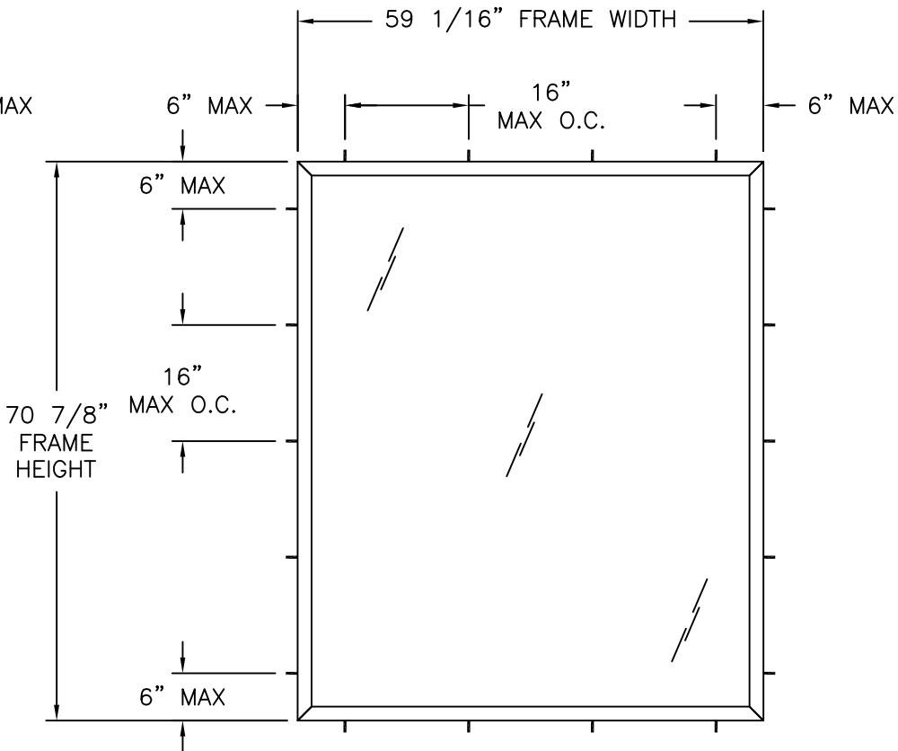
FLAT CLIP OR ANGLE ANCHORING FOR ALL RATINGS
