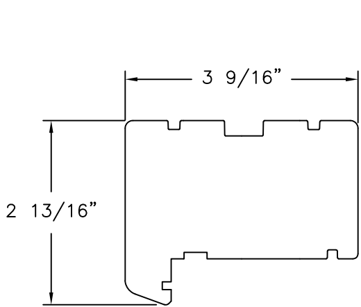
HEAD AND JAMB 3-4 LAYER OF CROSS GRAINED SOLID WOOD
