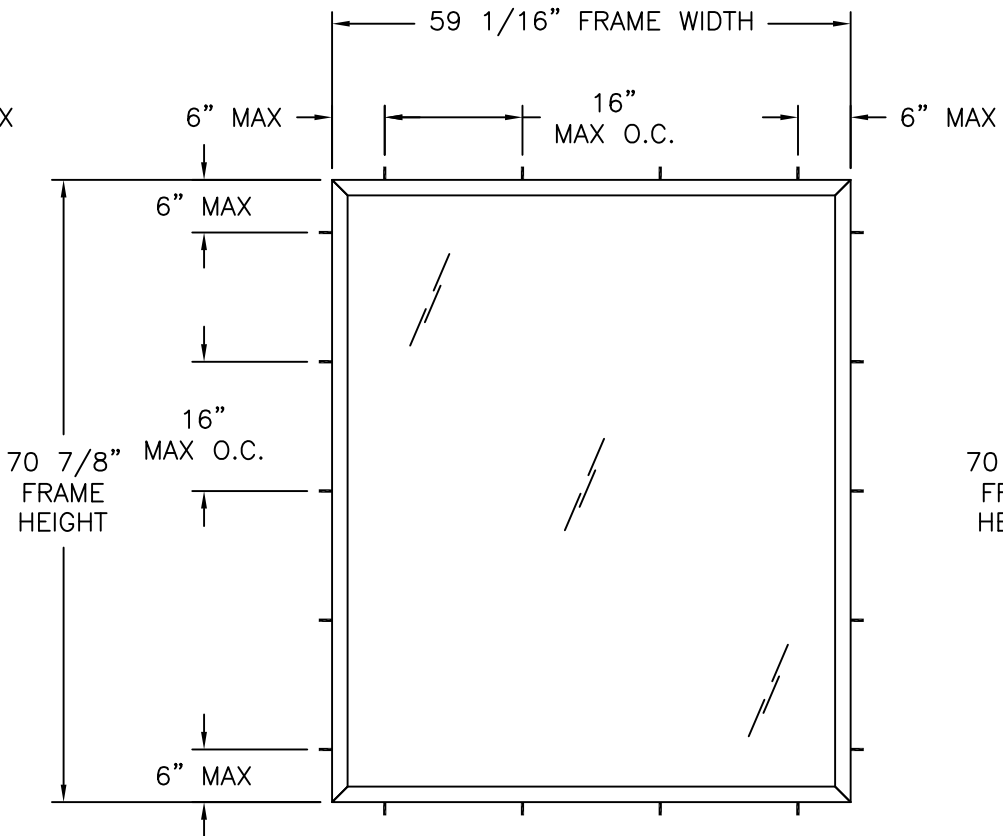
THROUGH FRAME ANCHORING FOR DP RATINGS LOWER THAN 30.0PSF
