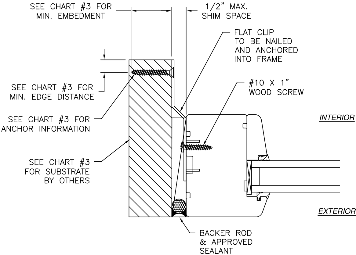
JAMB INSTALLATION DETAIL
