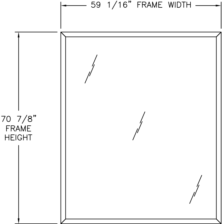
NW FIXED 510 WOOD WINDOW EXTERIOR VIEW
