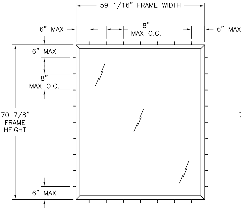
THROUGH FRAME ANCHORING FOR DP RATINGS 30.0PSF OR HIGHER
