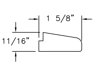
GLAZING BEAD SOLID WOOD
