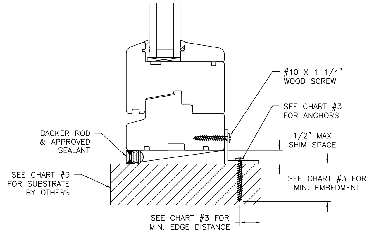
VERTICAL CROSS SECTION
