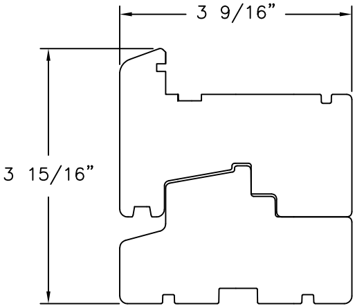
SILL 3-4 LAYER OF CROSS GRAINED SOLID WOOD
