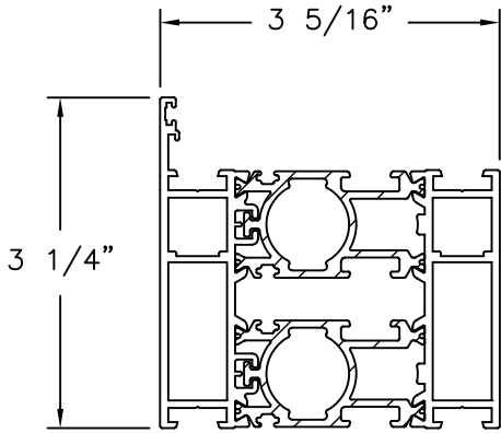
FRAME ALUMINUM 6063-T5 (.079" THICK)
