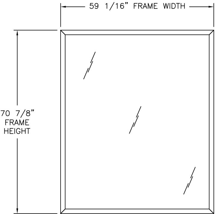
NW FIXED 810 ALUMINUM WINDOW EXTERIOR VIEW
