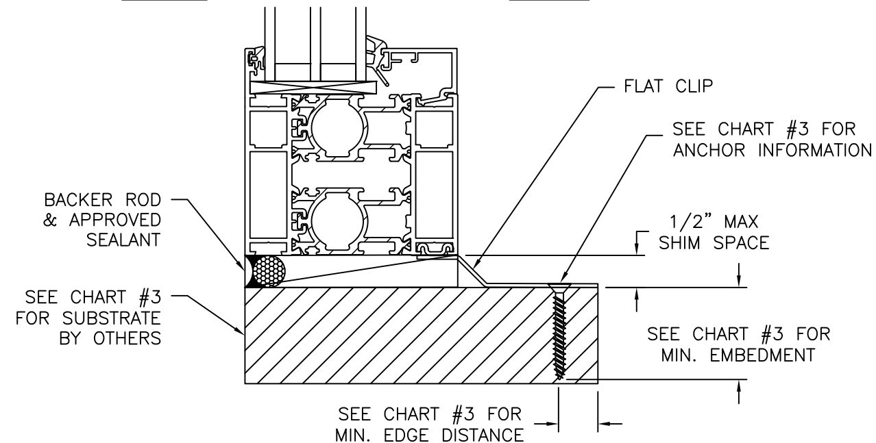
VERTICAL CROSS SECTION
