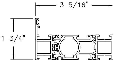
ALTERNATE FRAME ALUMINUM 6063-T5 (.079" THICK)
