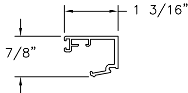
GLASS STOP ALUMINUM 6063-T5 (.067" THICK)
