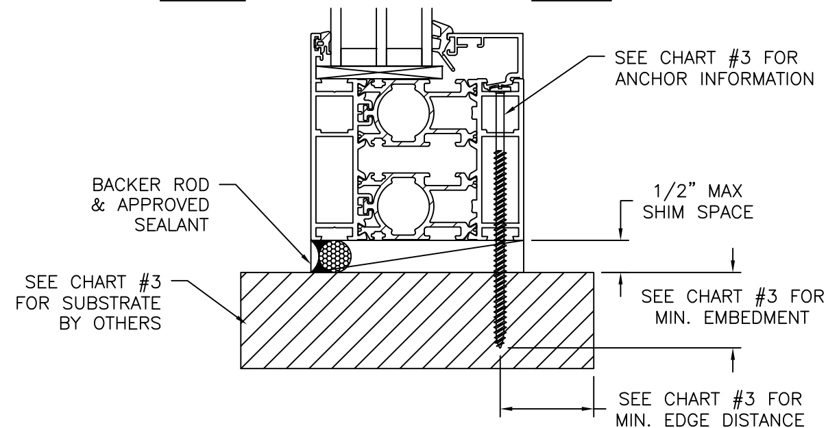
VERTICAL CROSS SECTION
