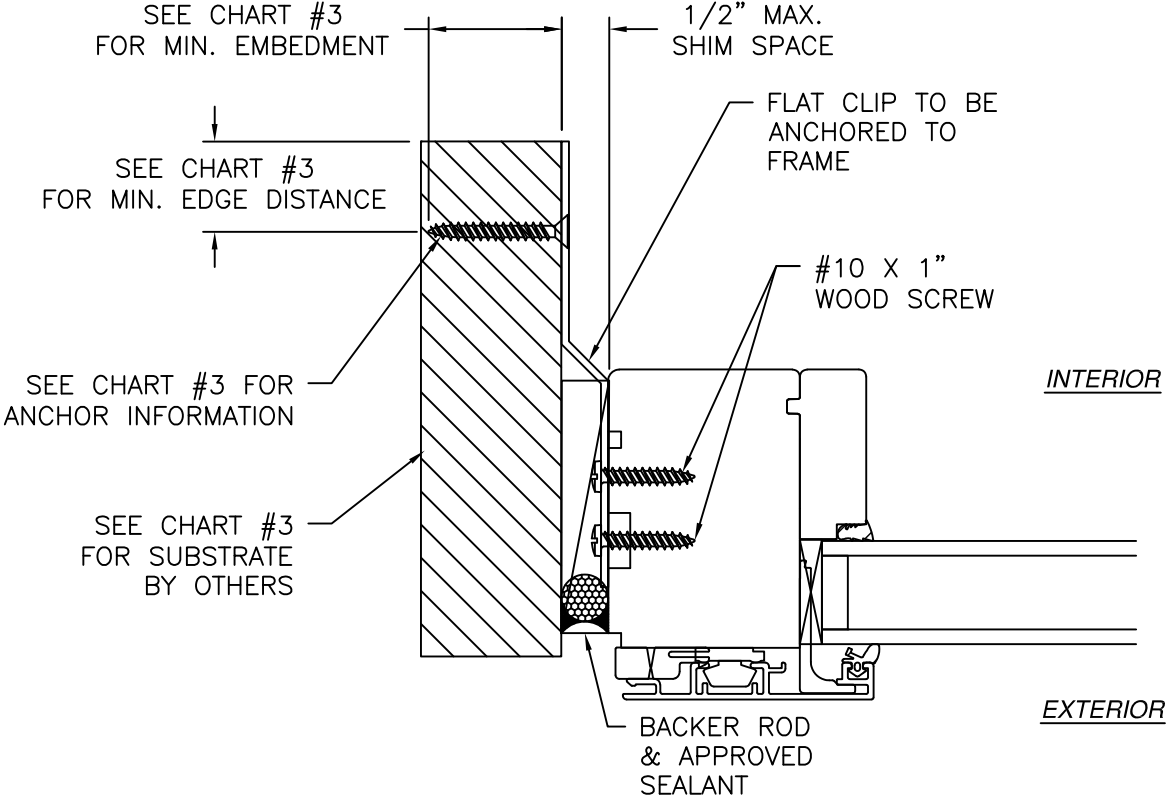
JAMB INSTALLATION DETAIL
