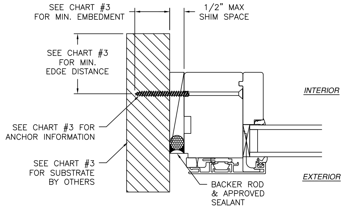
JAMB INSTALLATION DETAIL
