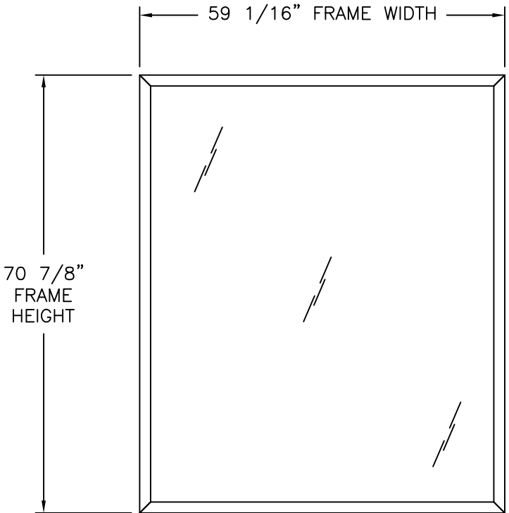
NW FIXED 710 WOOD WITH ALUMINUM CLAD WINDOW EXTERIOR VIEW
