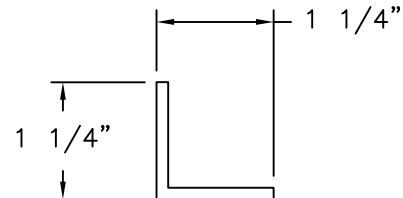
ANGLE CLIP 6063-T5 ALUMINUM (.125" THICK)
