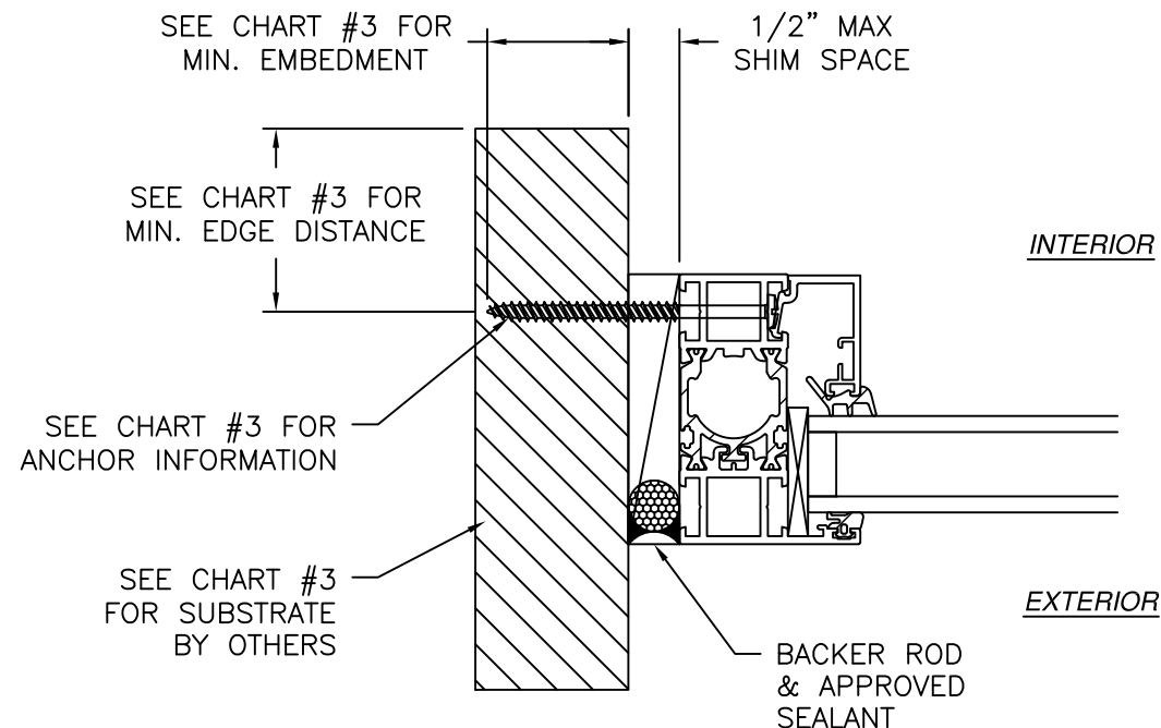
JAMB INSTALLATION DETAIL
