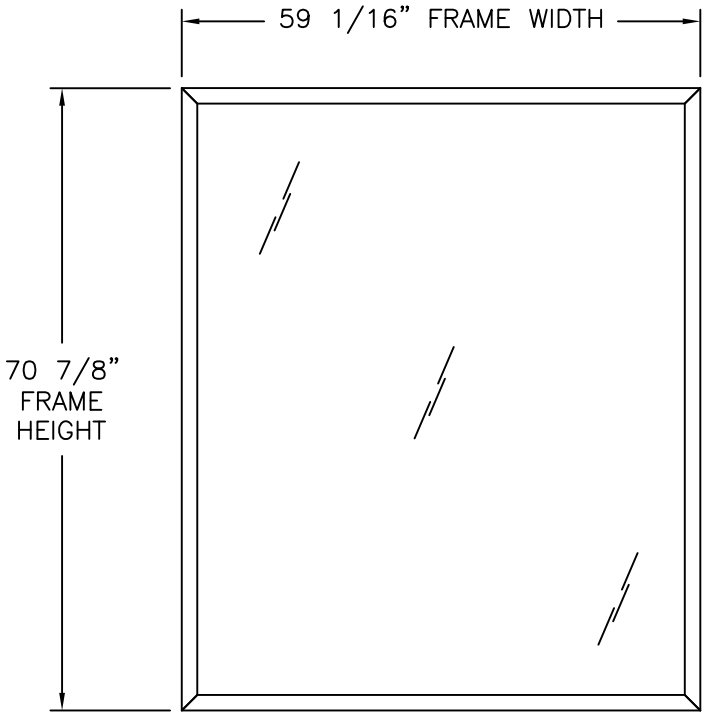
NW FIXED 610 ALUMINUM WINDOW EXTERIOR VIEW
