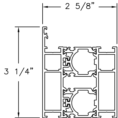
ALTERNATE FRAME ALUMINUM 6063-T5 (.079" THICK)
