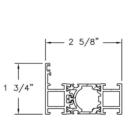
FRAME ALUMINUM 6063-T5 (.079" THICK)
