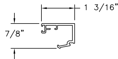
GLASS STOP ALUMINUM 6063-T5 (.067" THICK)
