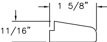
GLAZING BEAD SOLID WOOD
