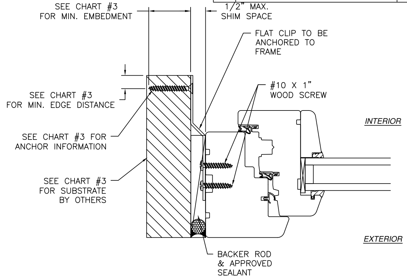
JAMB INSTALLATION DETAIL
