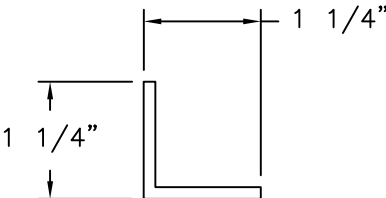
ANGLE CLIP 6063-T5 ALUMINUM (.125" THICK)
