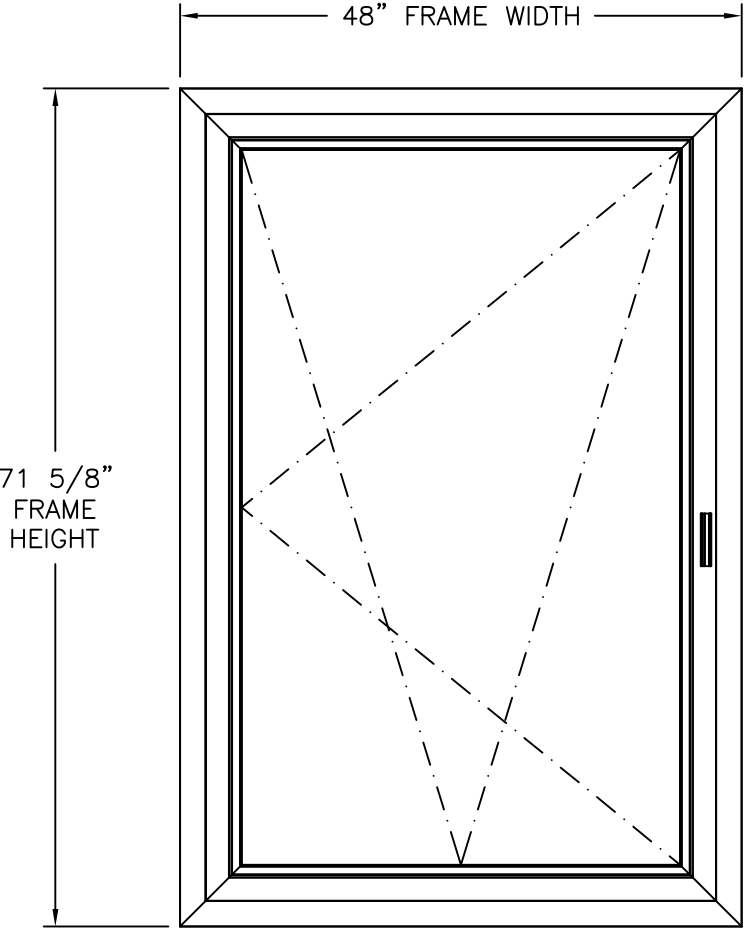
NW TILTTURN 820 ALUMINUM WINDOW EXTERIOR VIEW
