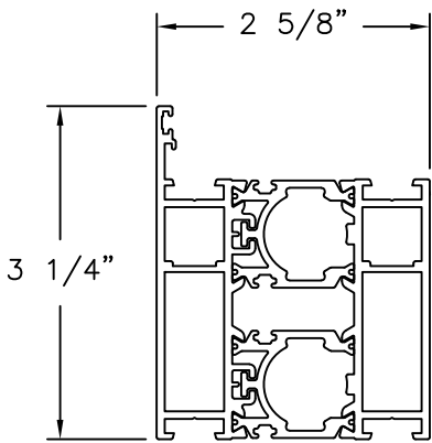
FRAME ALUMINUM 6063-T5 (.079" THICK)
