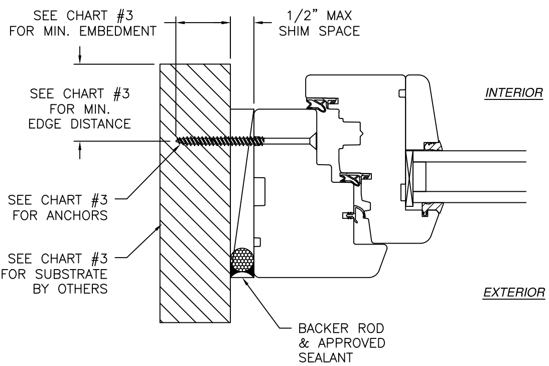
JAMB INSTALLATION DETAIL
