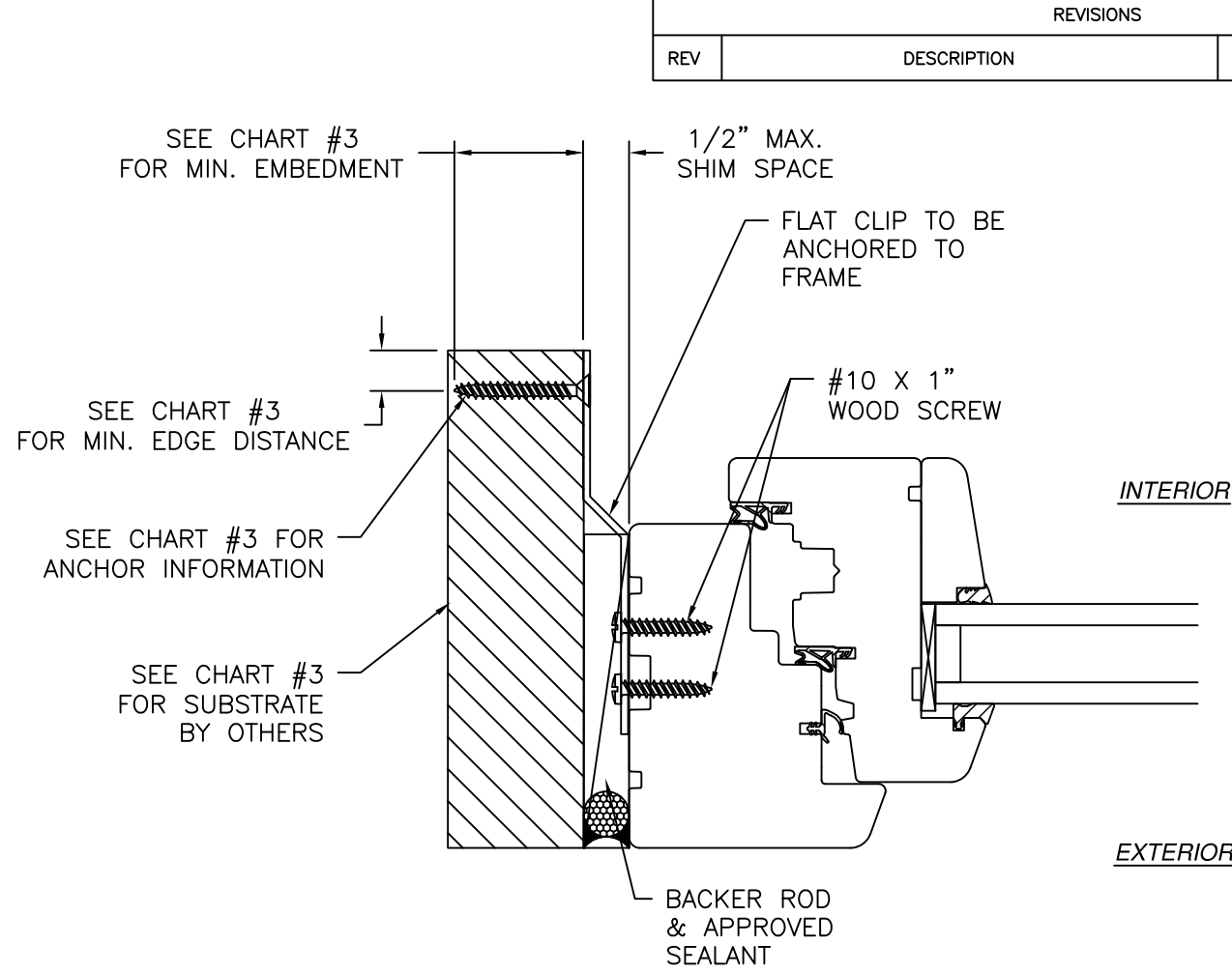
JAMB INSTALLATION DETAIL
