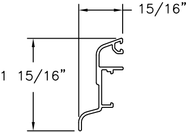
SILL EXTENDER ALUMINUM 6063-T5
