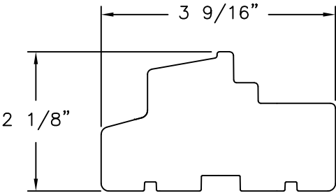
SILL 3-4 LAYER OF CROSS GRAINED SOLID WOOD
