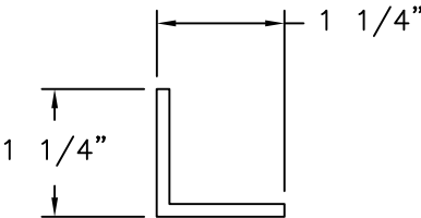
ANGLE CLIP 6063-T5 ALUMINUM (.125" THICK)
