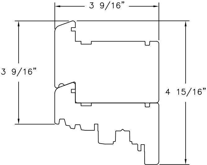
ALTERNATE SASH 3-4 LAYER OF CROSS GRAINED SOLID WOOD
