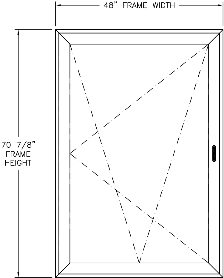
NW TILTTURN 520 WOOD WINDOW EXTERIOR VIEW
