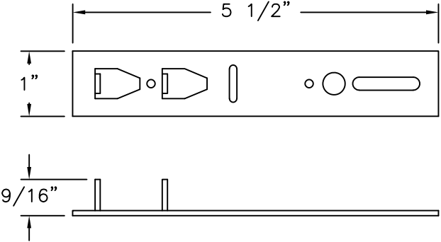
FLAT CLIP GALVANIZED STEEL (.058" THICK)
