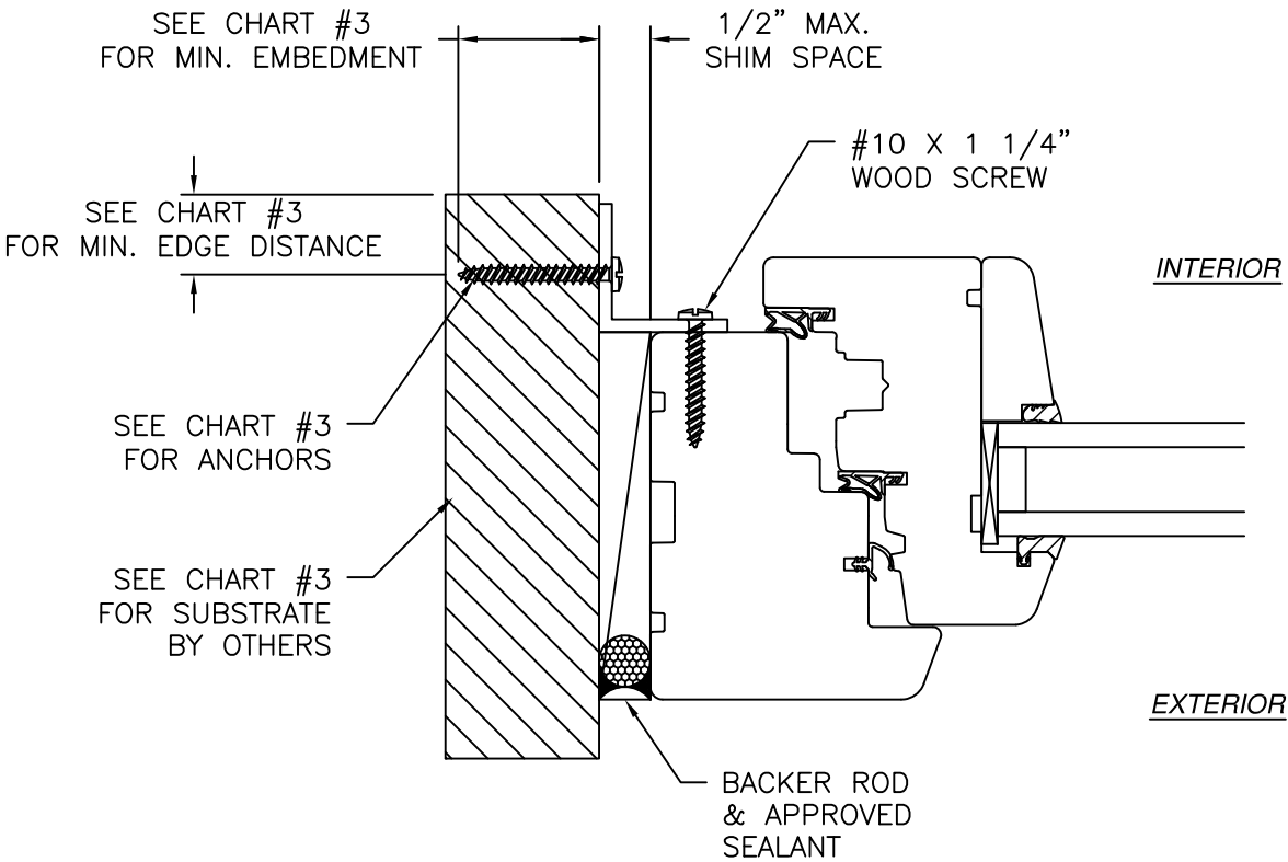
JAMB INSTALLATION DETAIL
