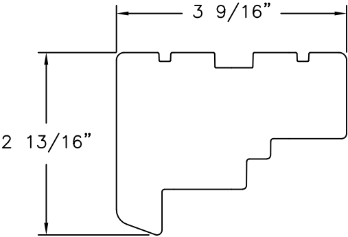
HEAD AND JAMB 3-4 LAYER OF CROSS GRAINED SOLID WOOD
