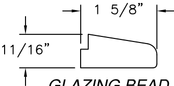
GLAZING BEAD SOLID WOOD
