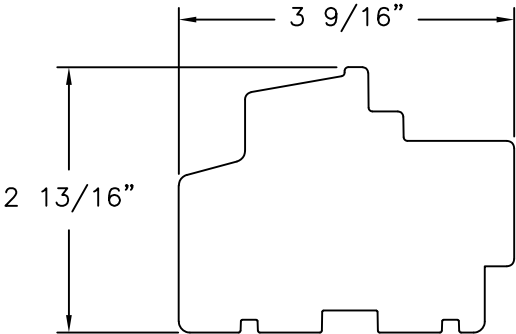
ALTERNATE SILL 3-4 LAYER OF CROSS GRAINED SOLID WOOD
