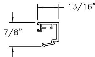
GLASS STOP ALUMINUM 6063-T5 (.067" THICK)
