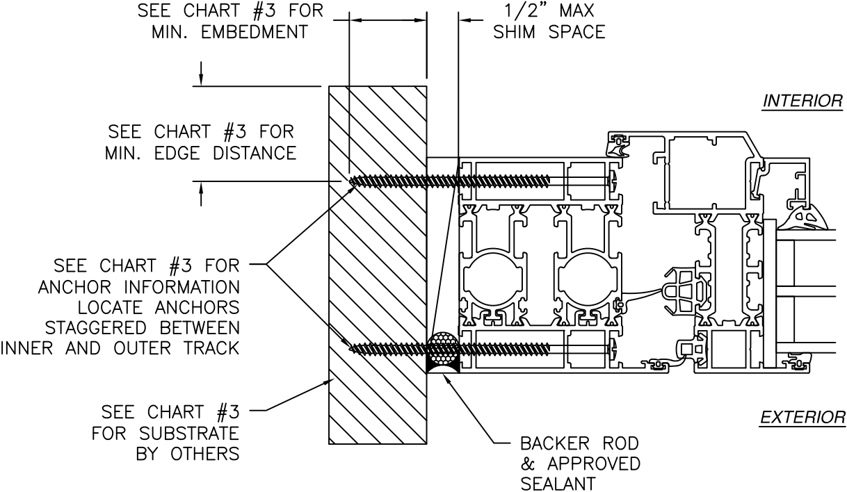
JAMB INSTALLATION DETAIL
