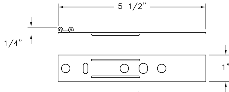
FLAT CLIP GALVANIZED STEEL (.058" THICK)
