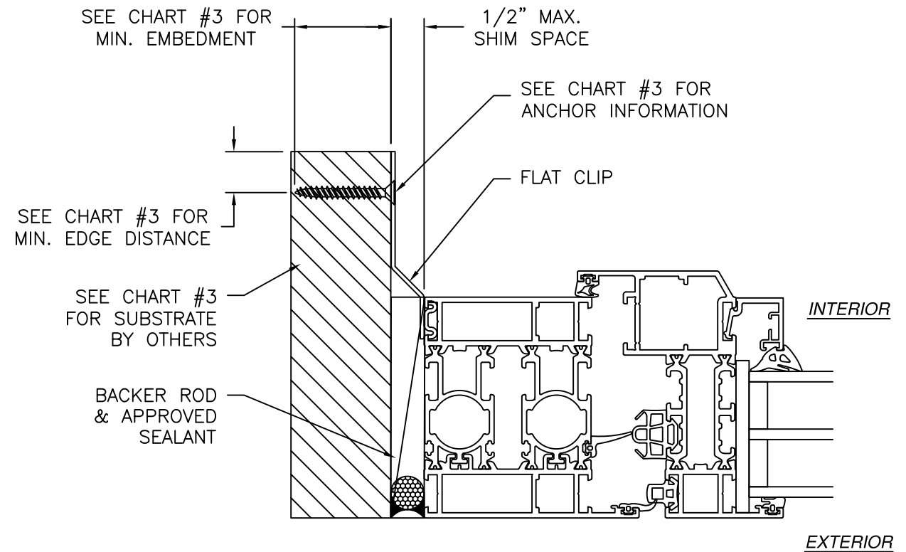
JAMB INSTALLATION DETAIL
