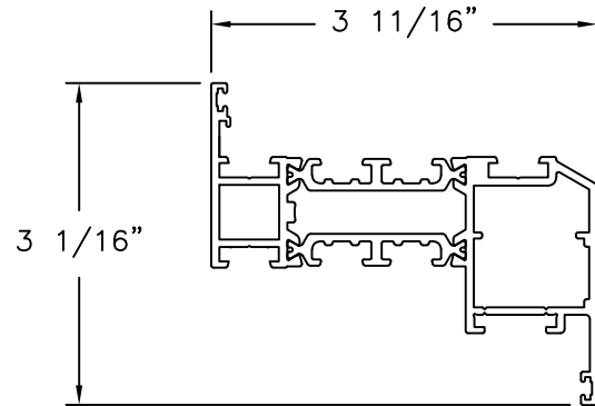
PANEL ALUMINUM 6063-T5 (.079" THICK)
