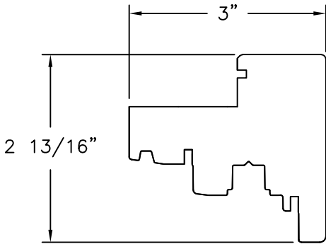
PANEL 3-4 LAYER OF CROSS GRAINED SOLID WOOD
