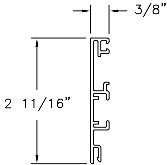
EXTERIOR COVER ALUMINUM 6063-T5
