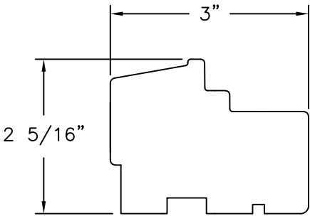
SILL 3-4 LAYER OF CROSS GRAINED SOLID WOOD
