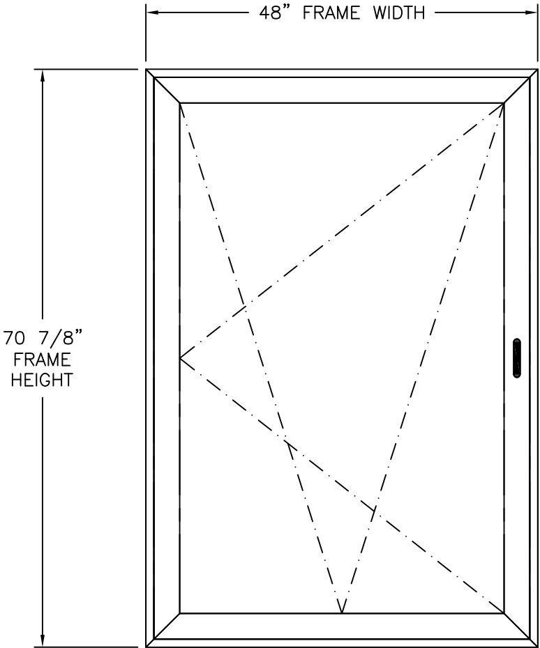
NW TILTTURN 720 WOOD WITH ALUMINUM CLAD WINDOW
