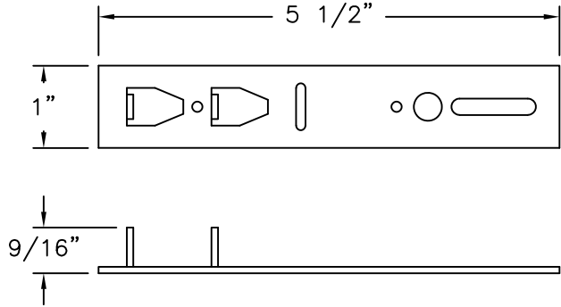
FLAT CLIP GALVANIZED STEEL (.058" THICK)
