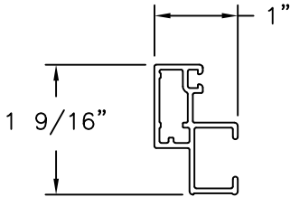
GLAZING BEAD ALUMINUM 6063-T5
