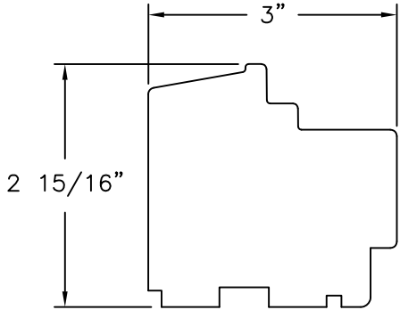
ALTERNATE SILL 3-4 LAYER OF CROSS GRAINED SOLID WOOD
