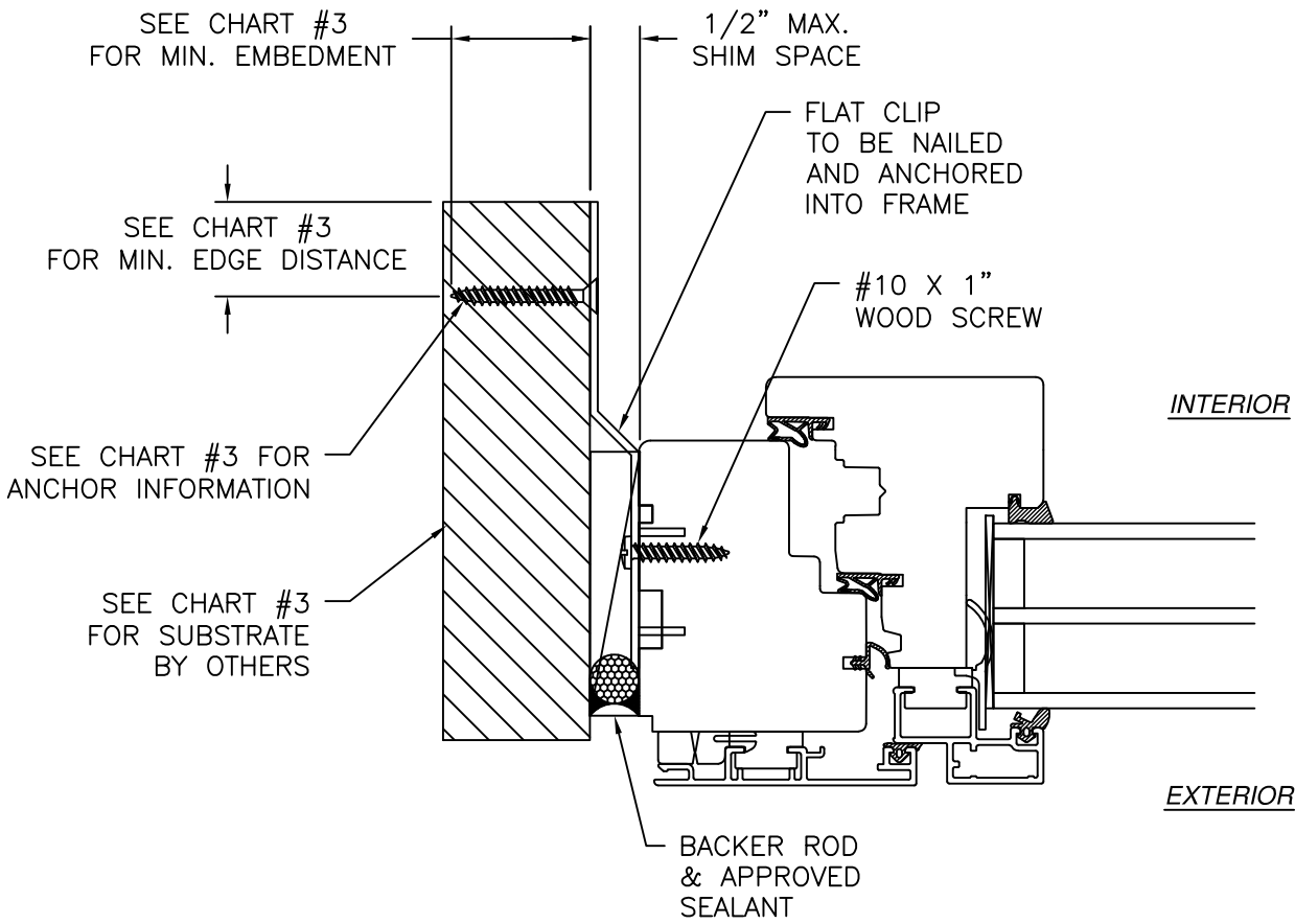
JAMB INSTALLATION DETAIL
